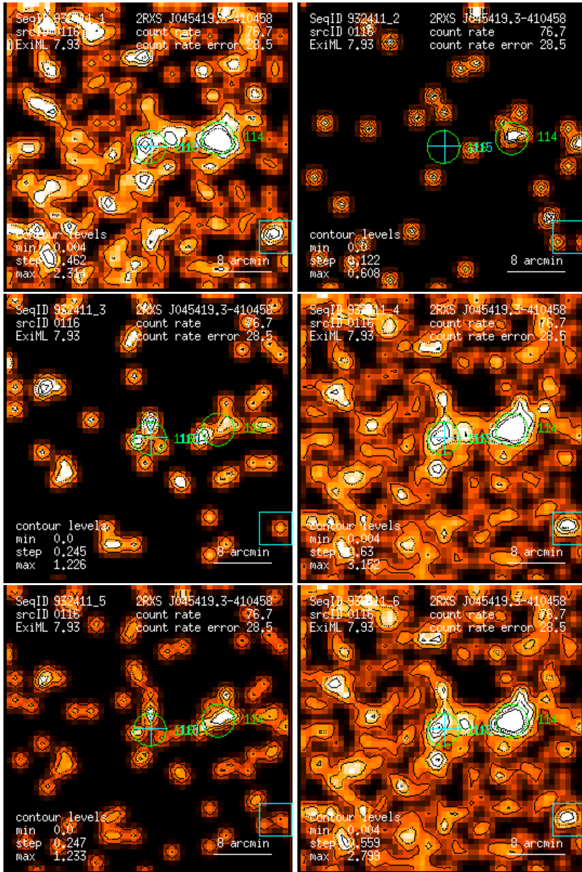
Figure 116: RASS 932411: detection 0116: band rate images, Gaussian filter: (1) PSPC channels 11 – 41, (2) 52 – 90, (3) 91 – 201, (4) 11 – 235, (5) 52 – 201, (6) 11 – 201. Broad band rates in counts/ks. Band rate contour levels in counts/ks/arcmin 2 .
