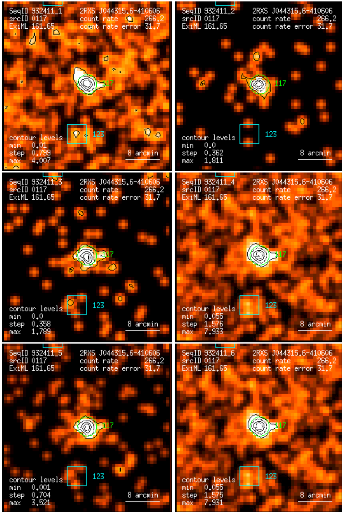
Figure 117: RASS 932411: detection 0117: band rate images, Gaussian filter: (1) PSPC channels 11 – 41, (2) 52 – 90, (3) 91 – 201, (4) 11 – 235, (5) 52 – 201, (6) 11 – 201. Broad band rates in counts/ks. Band rate contour levels in counts/ks/arcmin 2 .
