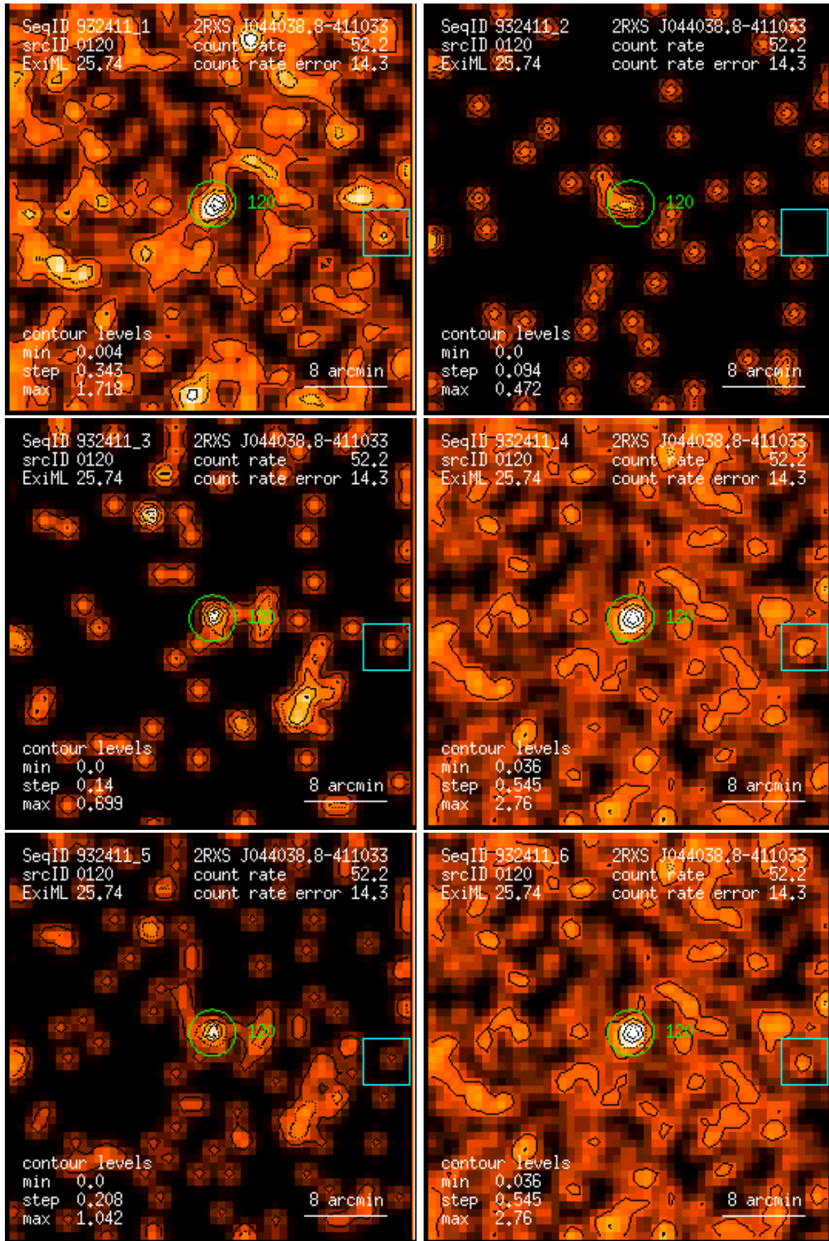
Figure 120: RASS 932411: detection 0120: band rate images, Gaussian filter: (1) PSPC channels 11 – 41, (2) 52 – 90, (3) 91 – 201, (4) 11 – 235, (5) 52 – 201, (6) 11 – 201. Broad band rates in counts/ks. Band rate contour levels in counts/ks/arcmin 2 .
