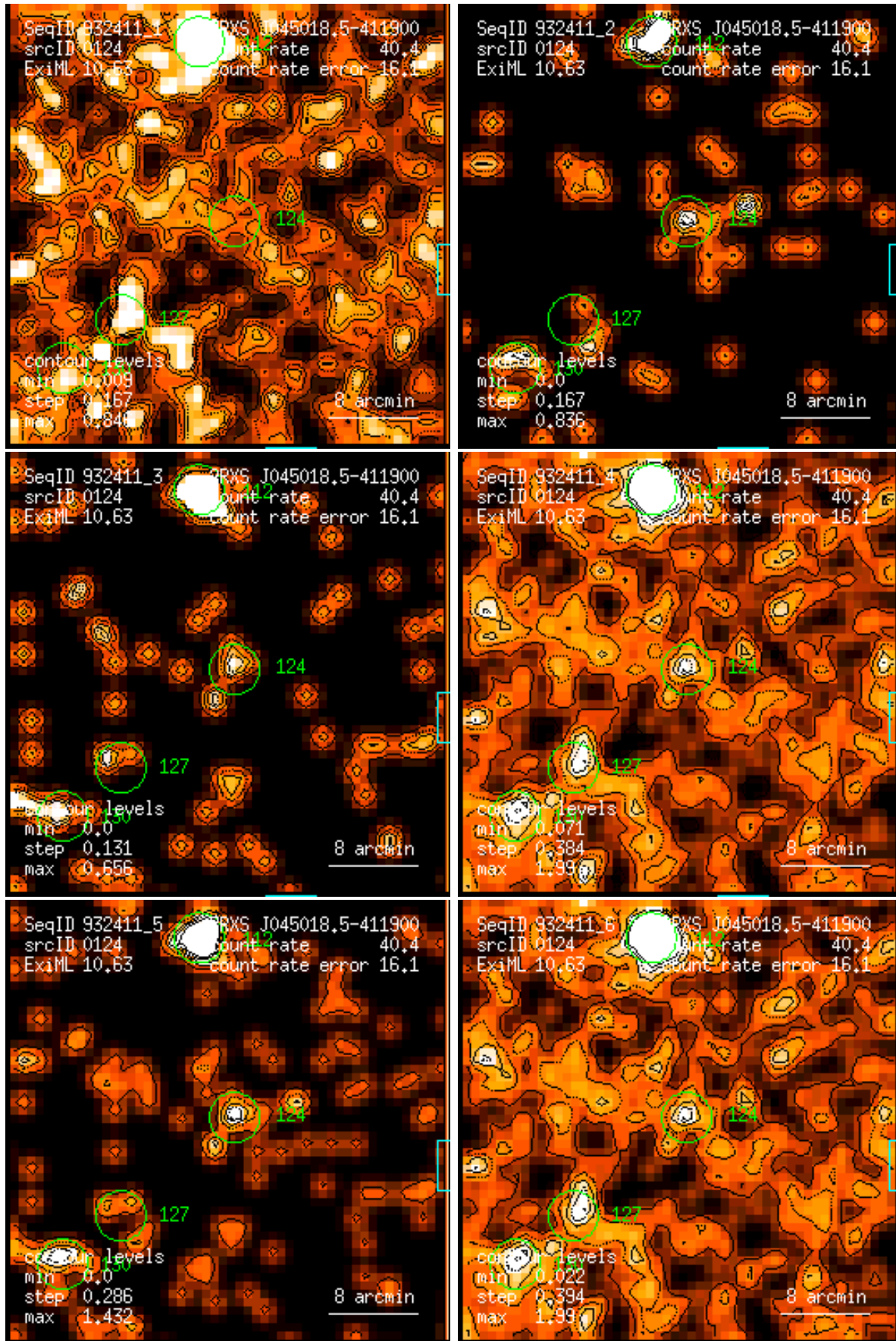
Figure 124: RASS 932411: detection 0124: band rate images, Gaussian filter: (1) PSPC channels 11 – 41, (2) 52 – 90, (3) 91 – 201, (4) 11 – 235, (5) 52 – 201, (6) 11 – 201. Broad band rates in counts/ks. Band rate contour levels in counts/ks/arcmin 2 .
