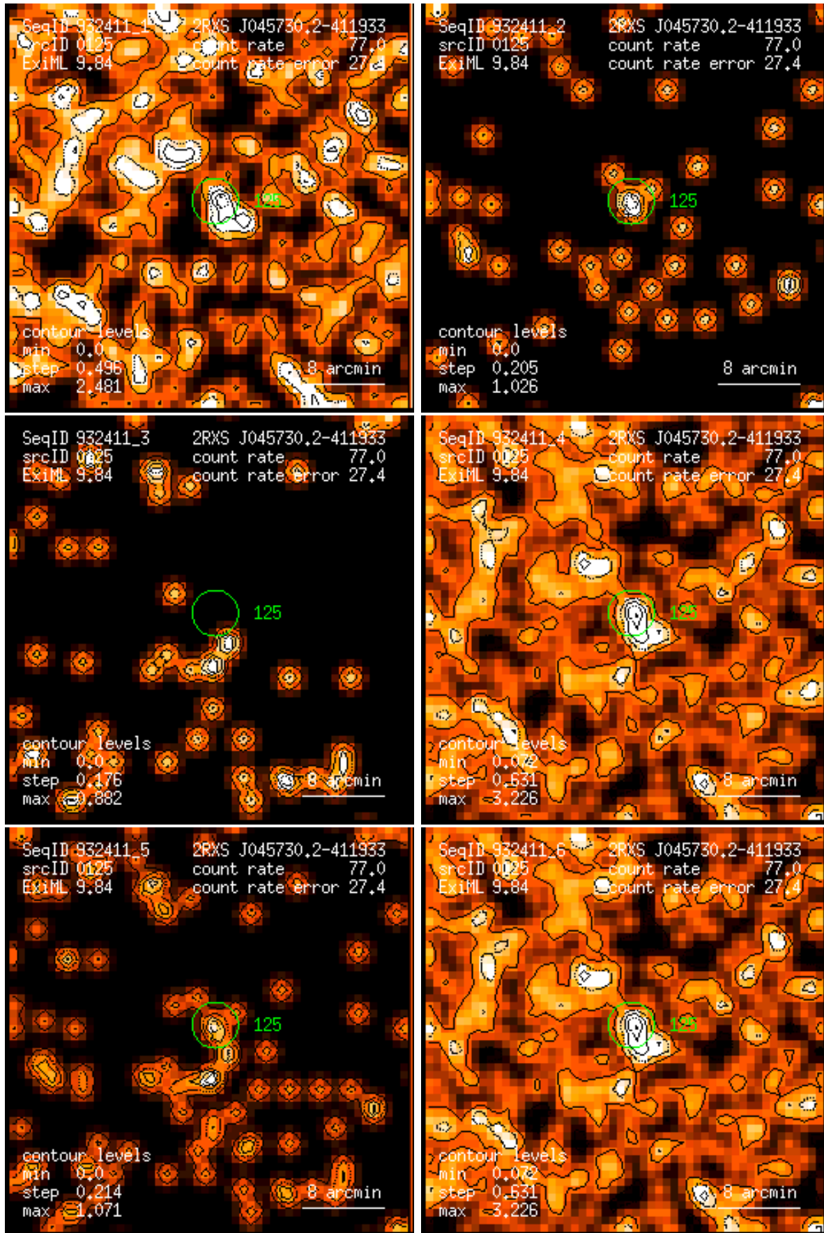
Figure 125: RASS 932411: detection 0125: band rate images, Gaussian filter: (1) PSPC channels 11 – 41, (2) 52 – 90, (3) 91 – 201, (4) 11 – 235, (5) 52 – 201, (6) 11 – 201. Broad band rates in counts/ks. Band rate contour levels in counts/ks/arcmin 2 .
