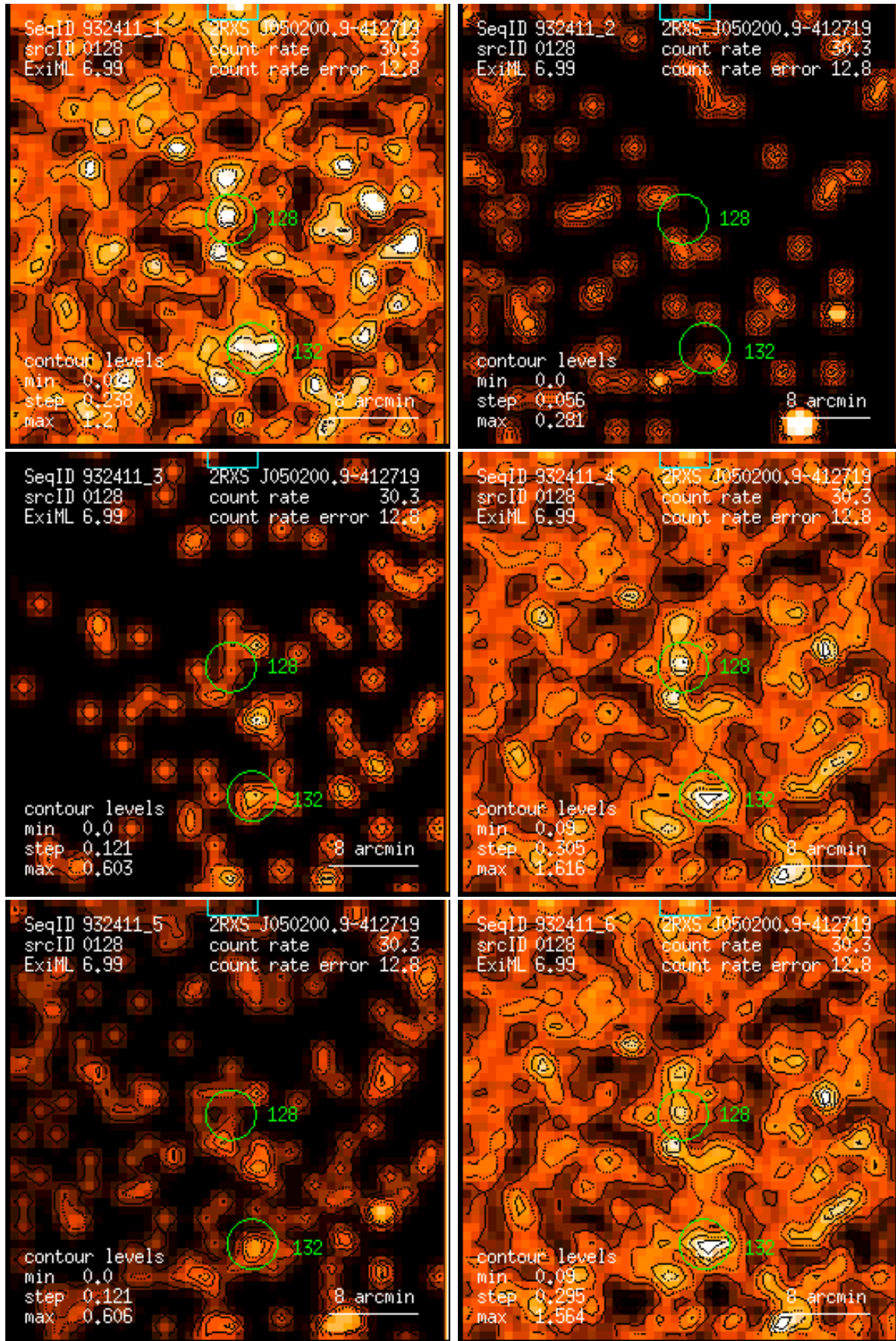
Figure 128: RASS 932411: detection 0128: band rate images, Gaussian filter: (1) PSPC channels 11 – 41, (2) 52 – 90, (3) 91 – 201, (4) 11 – 235, (5) 52 – 201, (6) 11 – 201. Broad band rates in counts/ks. Band rate contour levels in counts/ks/arcmin 2 .
