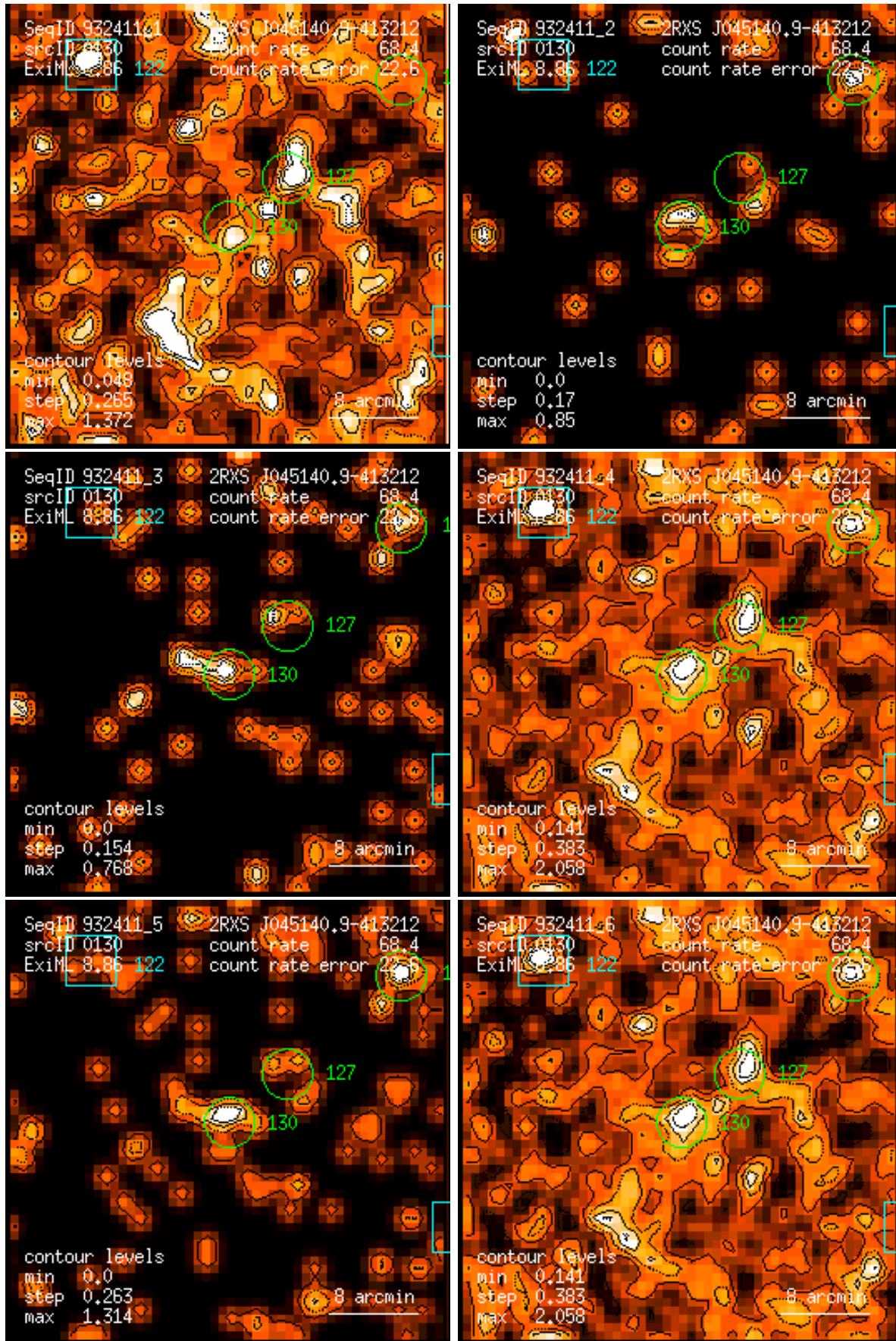
Figure 130: RASS 932411: detection 0130: band rate images, Gaussian filter: (1) PSPC channels 11 – 41, (2) 52 – 90, (3) 91 – 201, (4) 11 – 235, (5) 52 – 201, (6) 11 – 201. Broad band rates in counts/ks. Band rate contour levels in counts/ks/arcmin 2 .
