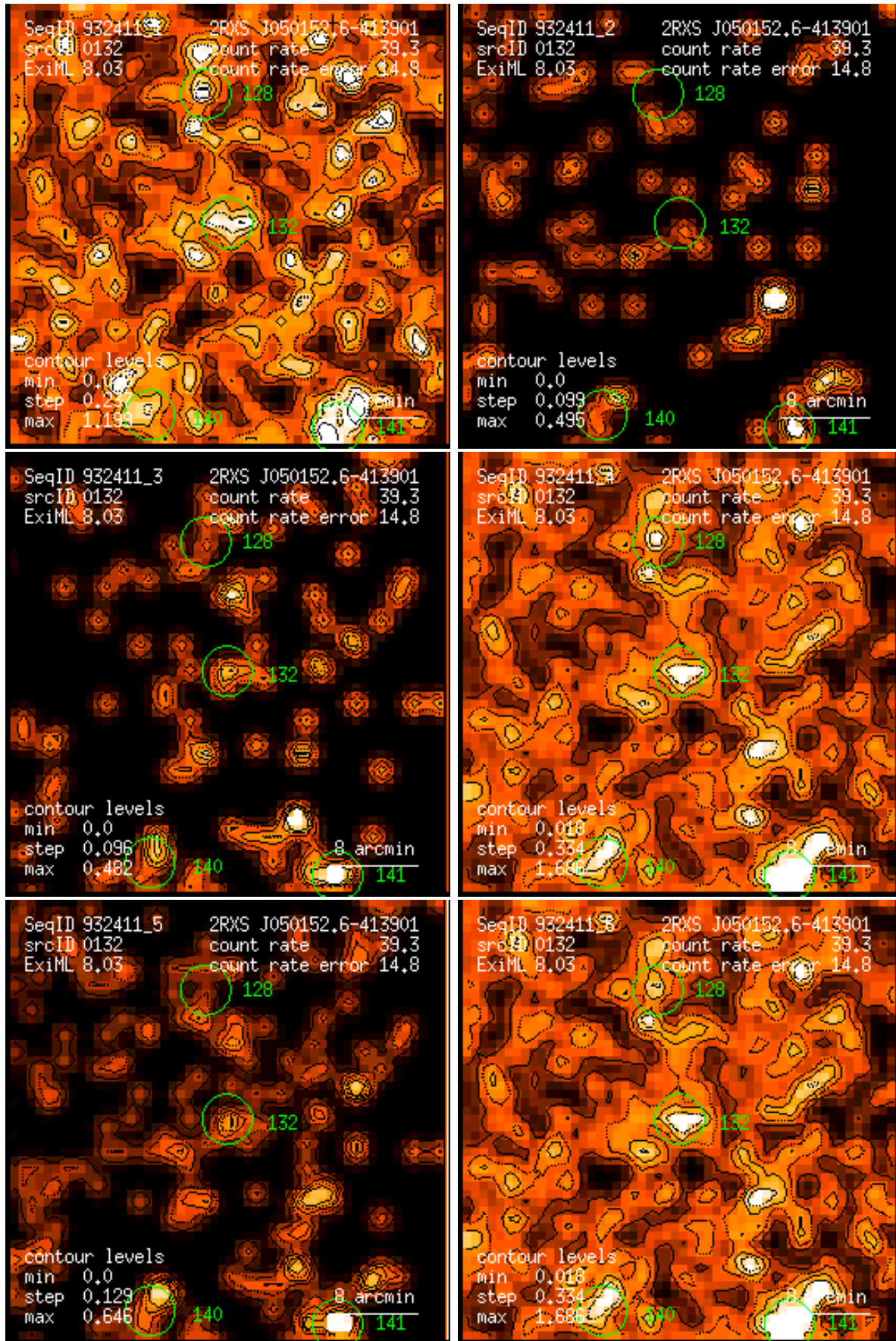
Figure 132: RASS 932411: detection 0132: band rate images, Gaussian filter: (1) PSPC channels 11 – 41, (2) 52 – 90, (3) 91 – 201, (4) 11 – 235, (5) 52 – 201, (6) 11 – 201. Broad band rates in counts/ks. Band rate contour levels in counts/ks/arcmin 2 .
