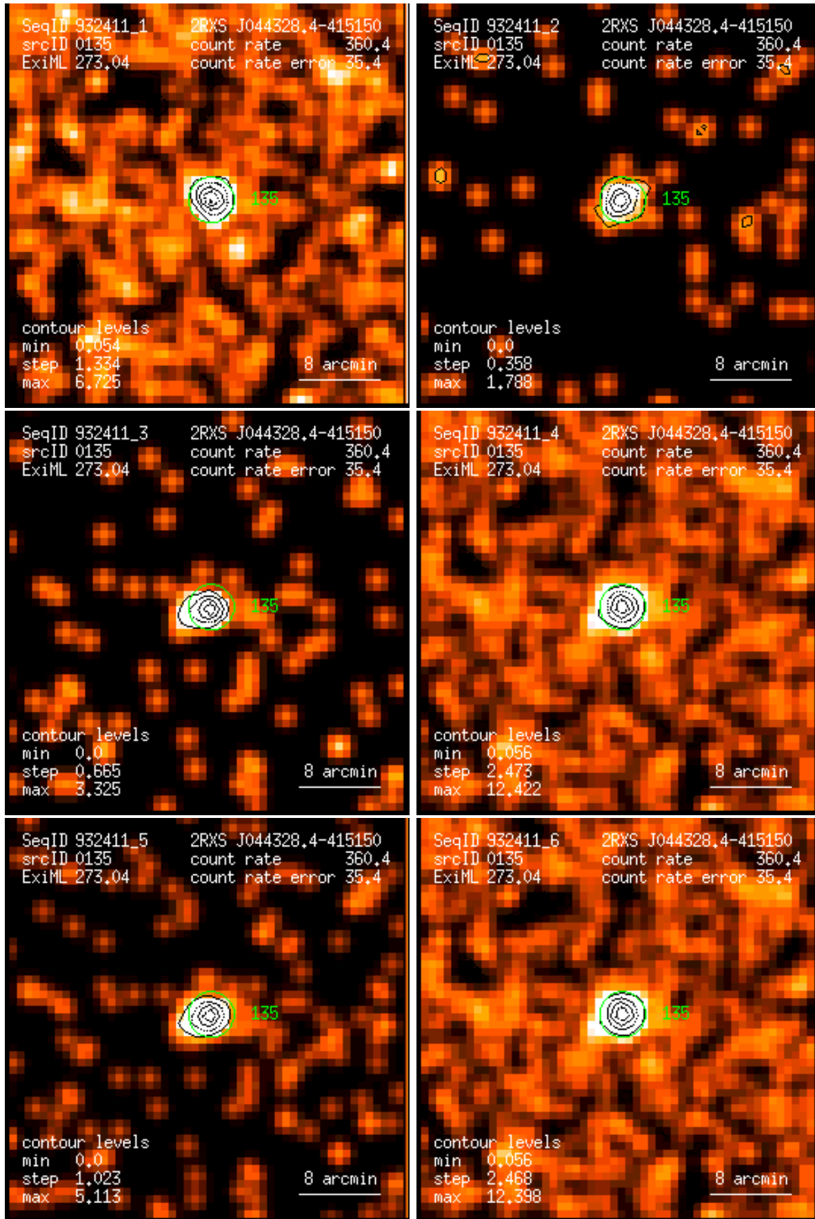
Figure 135: RASS 932411: detection 0135: band rate images, Gaussian filter: (1) PSPC channels 11 – 41, (2) 52 – 90, (3) 91 – 201, (4) 11 – 235, (5) 52 – 201, (6) 11 – 201. Broad band rates in counts/ks. Band rate contour levels in counts/ks/arcmin 2 .
