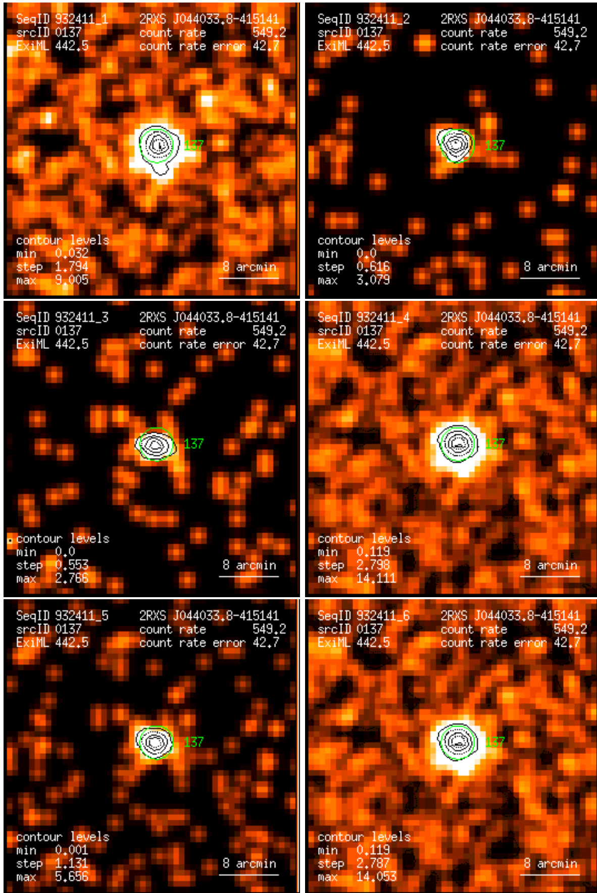
Figure 137: RASS 932411: detection 0137: band rate images, Gaussian filter: (1) PSPC channels 11 – 41, (2) 52 – 90, (3) 91 – 201, (4) 11 – 235, (5) 52 – 201, (6) 11 – 201. Broad band rates in counts/ks. Band rate contour levels in counts/ks/arcmin 2 .
