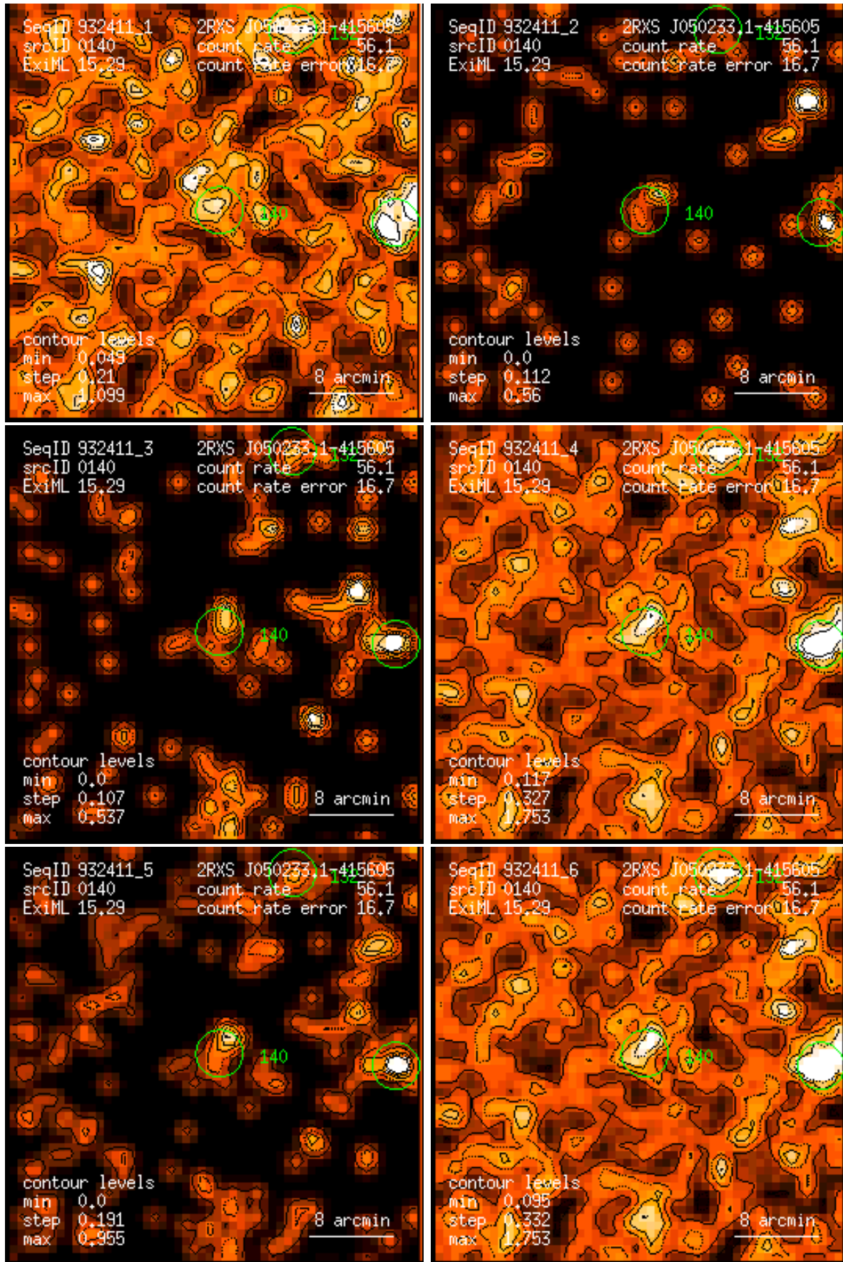
Figure 140: RASS 932411: detection 0140: band rate images, Gaussian filter: (1) PSPC channels 11 – 41, (2) 52 – 90, (3) 91 – 201, (4) 11 – 235, (5) 52 – 201, (6) 11 – 201. Broad band rates in counts/ks. Band rate contour levels in counts/ks/arcmin 2 .
