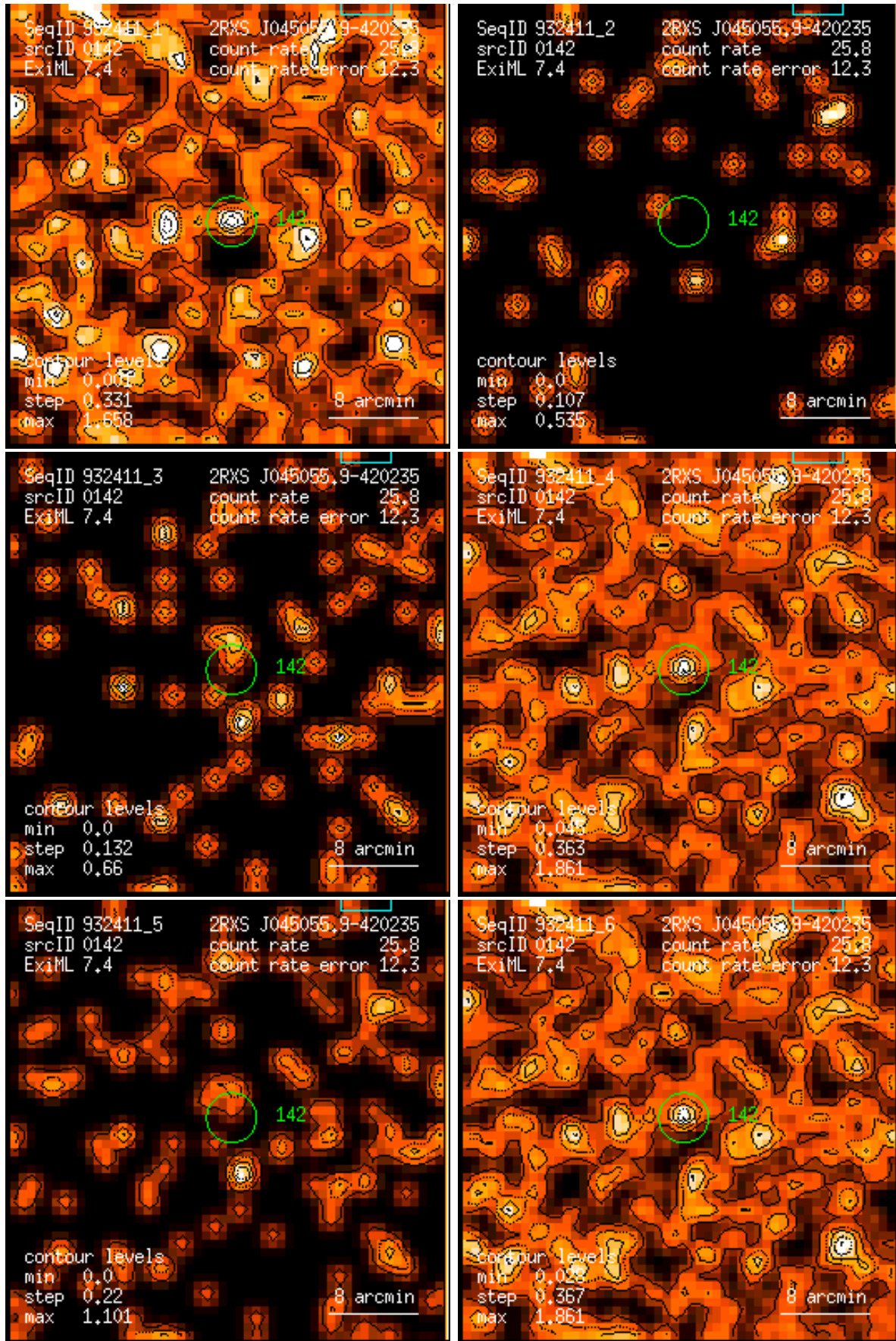
Figure 142: RASS 932411: detection 0142: band rate images, Gaussian filter: (1) PSPC channels 11 – 41, (2) 52 – 90, (3) 91 – 201, (4) 11 – 235, (5) 52 – 201, (6) 11 – 201. Broad band rates in counts/ks. Band rate contour levels in counts/ks/arcmin 2 .
