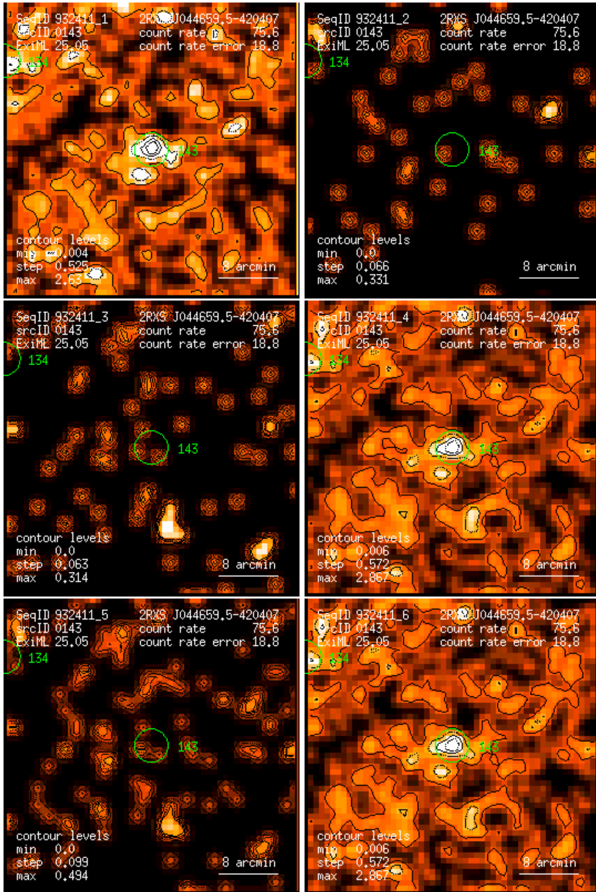
Figure 143: RASS 932411: detection 0143: band rate images, Gaussian filter: (1) PSPC channels 11 – 41, (2) 52 – 90, (3) 91 – 201, (4) 11 – 235, (5) 52 – 201, (6) 11 – 201. Broad band rates in counts/ks. Band rate contour levels in counts/ks/arcmin 2 .
