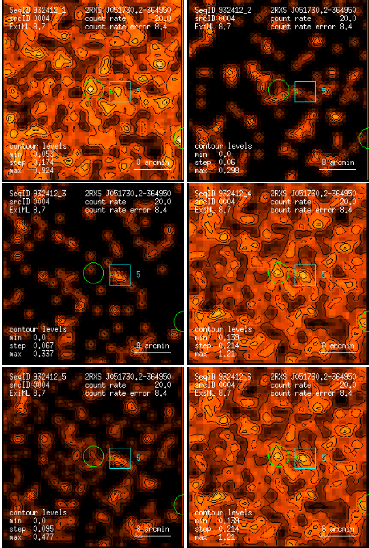
Figure 4: RASS 932412: detection 0004: band rate images, Gaussian filter: (1) PSPC channels 11 – 41, (2) 52 – 90, (3) 91 – 201, (4) 11 – 235, (5) 52 – 201, (6) 11 – 201. Broad band rates in counts/ks. Band rate contour levels in counts/ks/arcmin 2 .
