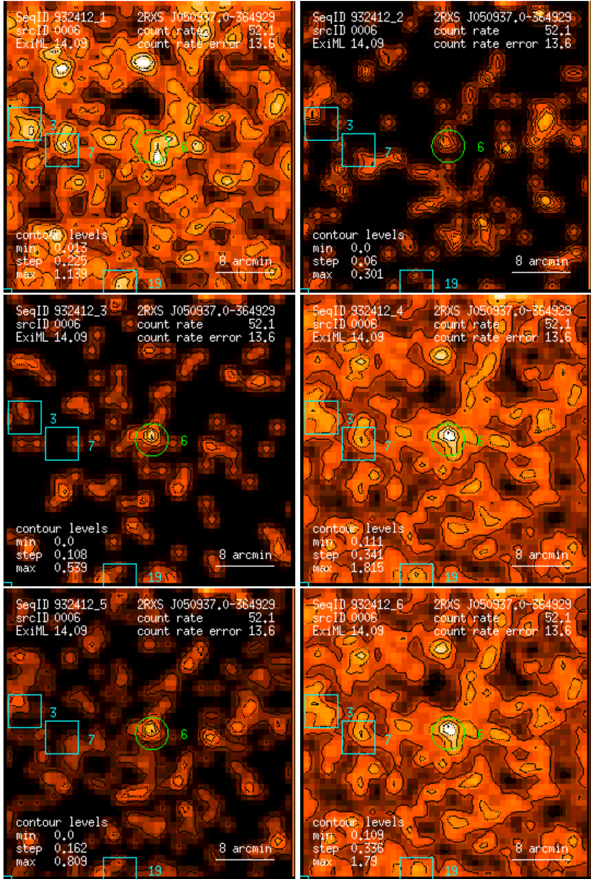
Figure 6: RASS 932412: detection 0006: band rate images, Gaussian filter: (1) PSPC channels 11 – 41, (2) 52 – 90, (3) 91 – 201, (4) 11 – 235, (5) 52 – 201, (6) 11 – 201. Broad band rates in counts/ks. Band rate contour levels in counts/ks/arcmin 2 .
