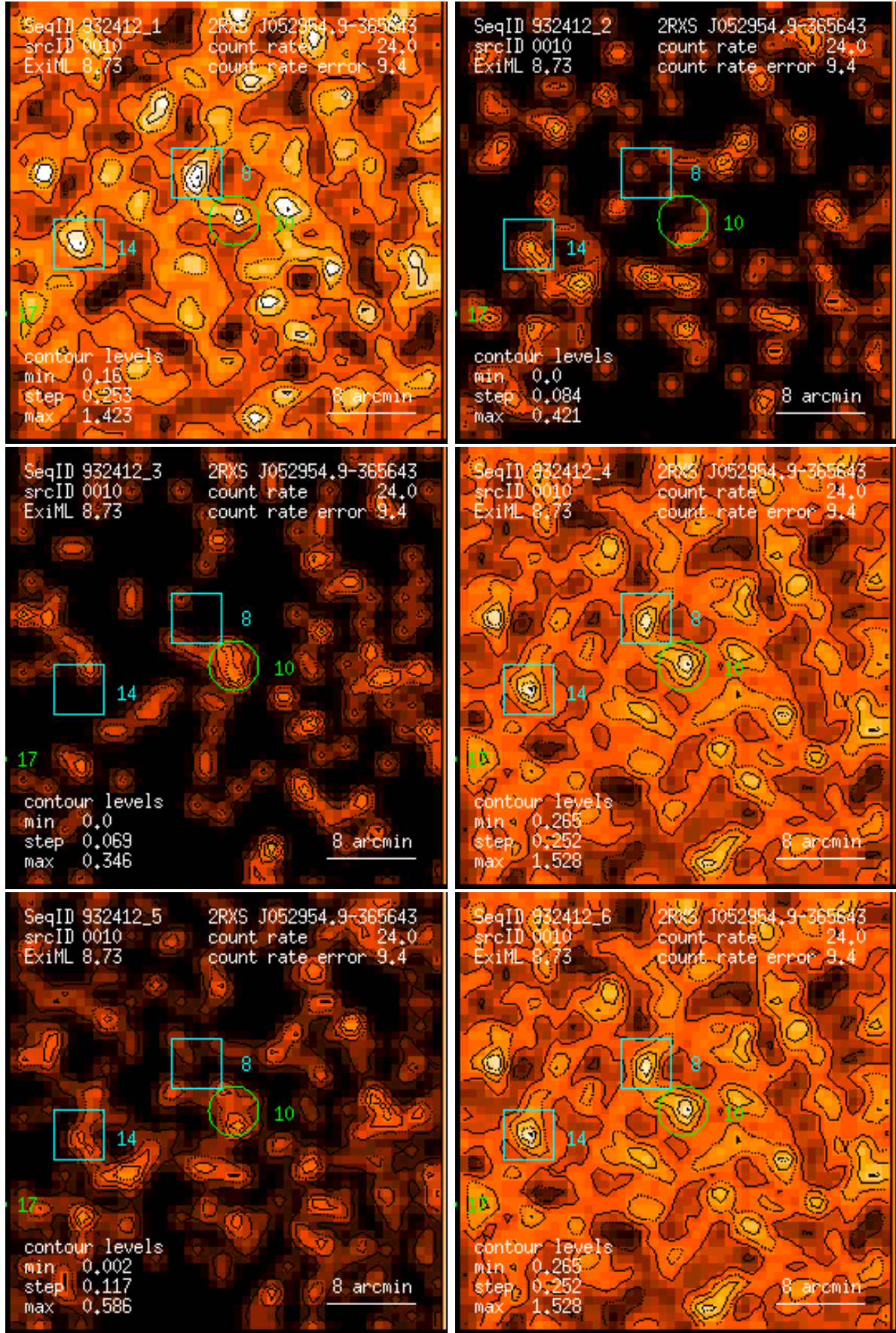
Figure 10: RASS 932412: detection 0010: band rate images, Gaussian filter: (1) PSPC channels 11 – 41, (2) 52 – 90, (3) 91 – 201, (4) 11 – 235, (5) 52 – 201, (6) 11 – 201. Broad band rates in counts/ks. Band rate contour levels in counts/ks/arcmin 2 .
