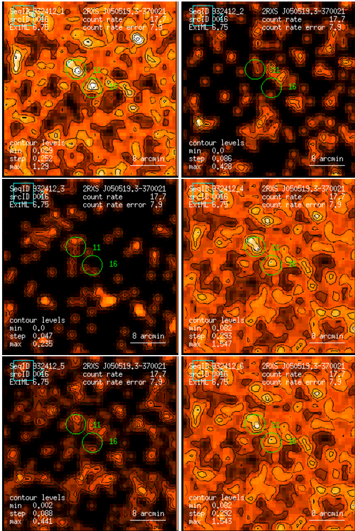
Figure 16: RASS 932412: detection 0016: band rate images, Gaussian filter: (1) PSPC channels 11 – 41, (2) 52 – 90, (3) 91 – 201, (4) 11 – 235, (5) 52 – 201, (6) 11 – 201. Broad band rates in counts/ks. Band rate contour levels in counts/ks/arcmin 2 .
