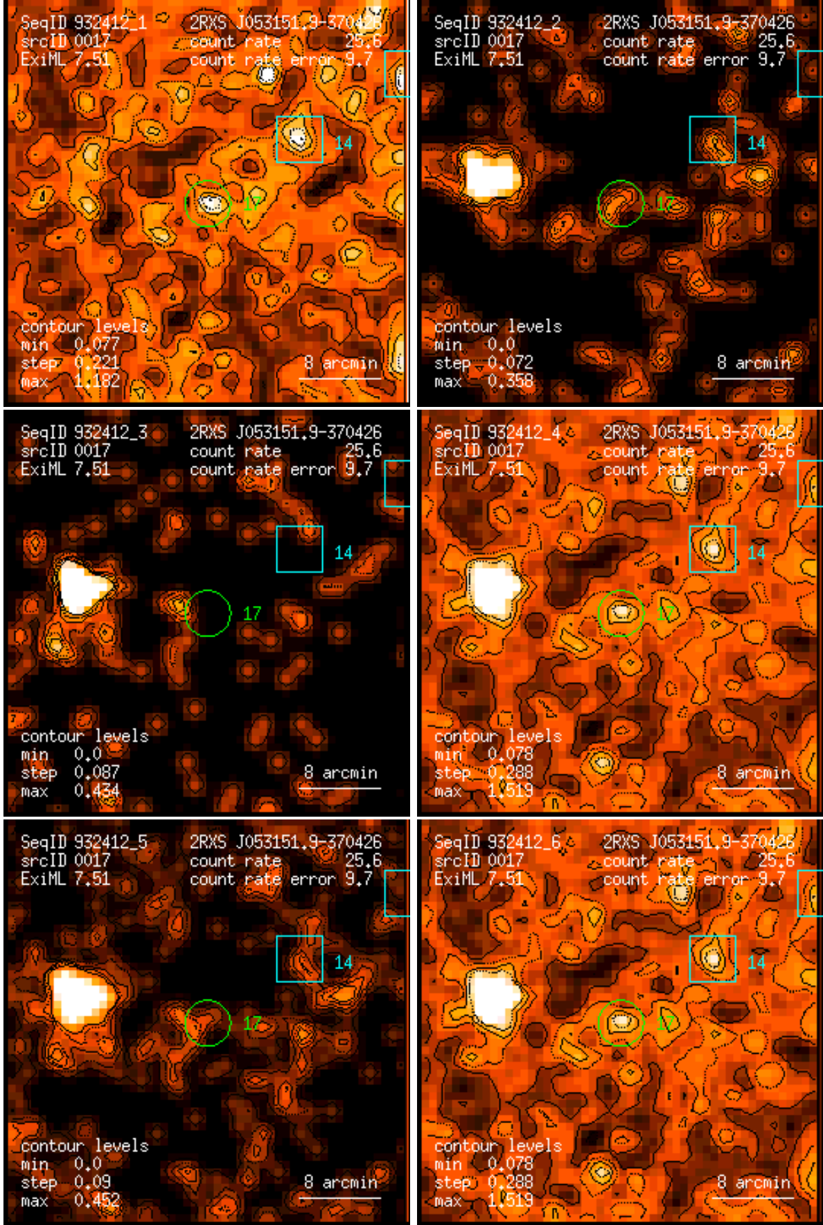
Figure 17: RASS 932412: detection 0017: band rate images, Gaussian filter: (1) PSPC channels 11 – 41, (2) 52 – 90, (3) 91 – 201, (4) 11 – 235, (5) 52 – 201, (6) 11 – 201. Broad band rates in counts/ks. Band rate contour levels in counts/ks/arcmin 2 .
