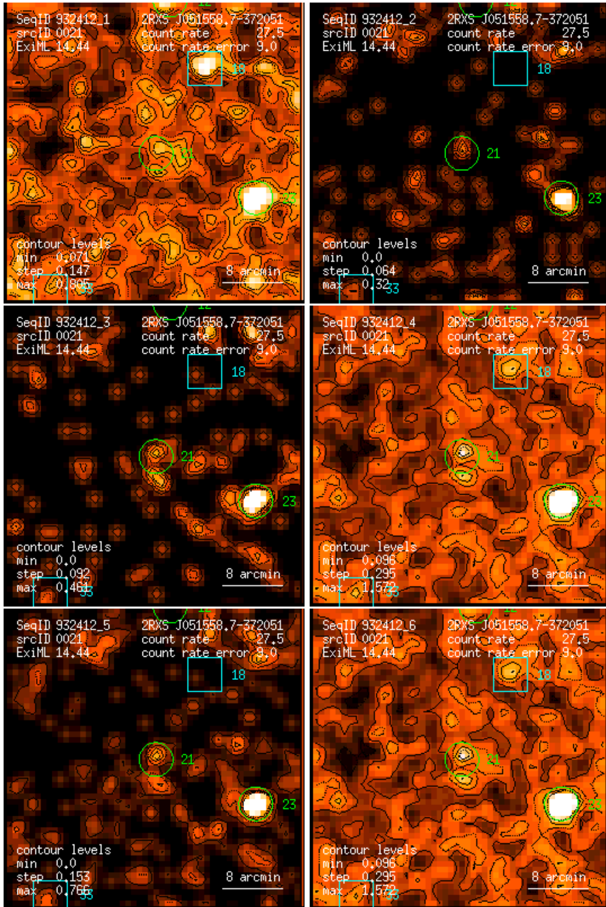
Figure 21: RASS 932412: detection 0021: band rate images, Gaussian filter: (1) PSPC channels 11 – 41, (2) 52 – 90, (3) 91 – 201, (4) 11 – 235, (5) 52 – 201, (6) 11 – 201. Broad band rates in counts/ks. Band rate contour levels in counts/ks/arcmin 2 .
