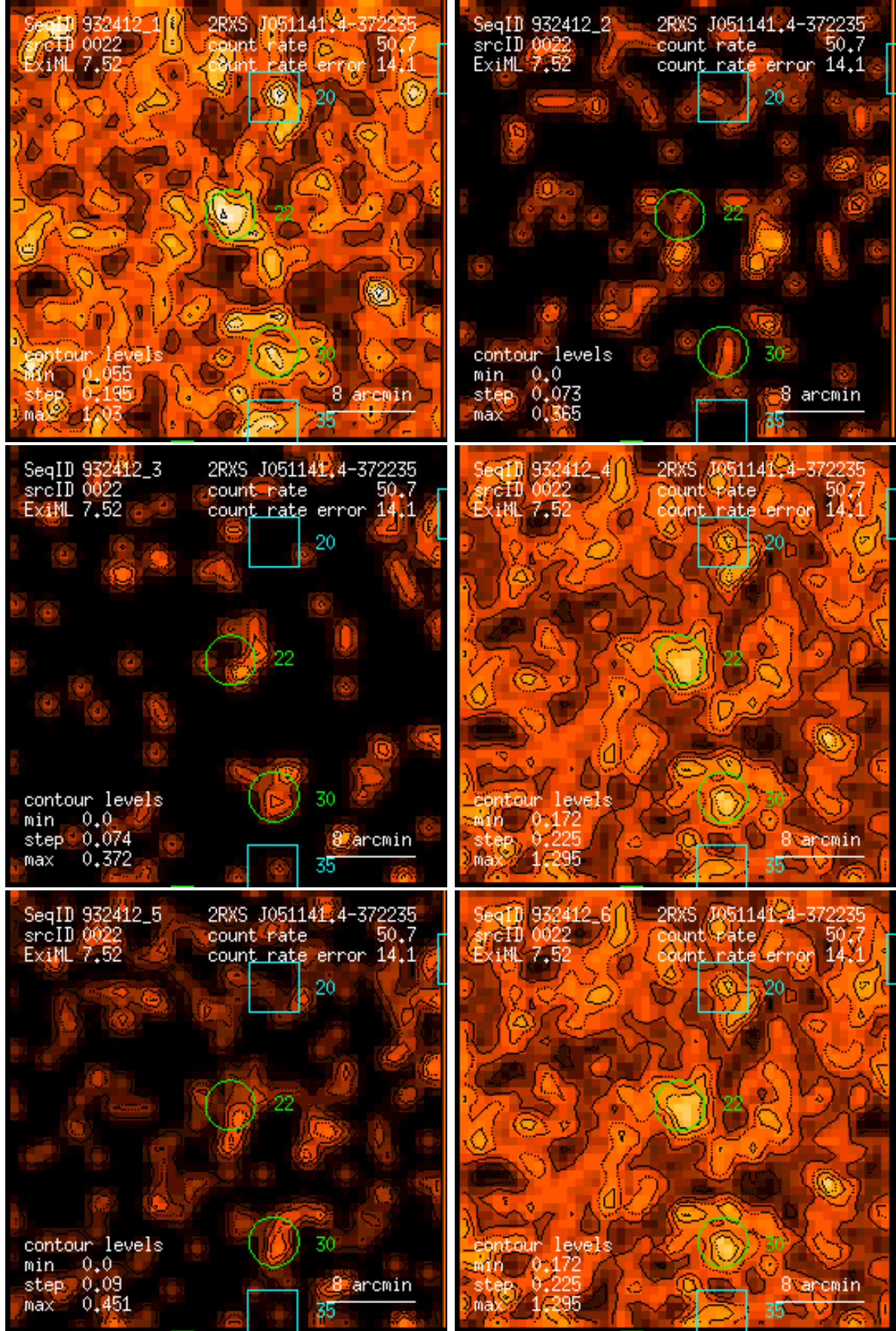
Figure 22: RASS 932412: detection 0022: band rate images, Gaussian filter: (1) PSPC channels 11 – 41, (2) 52 – 90, (3) 91 – 201, (4) 11 – 235, (5) 52 – 201, (6) 11 – 201. Broad band rates in counts/ks. Band rate contour levels in counts/ks/arcmin 2 .
