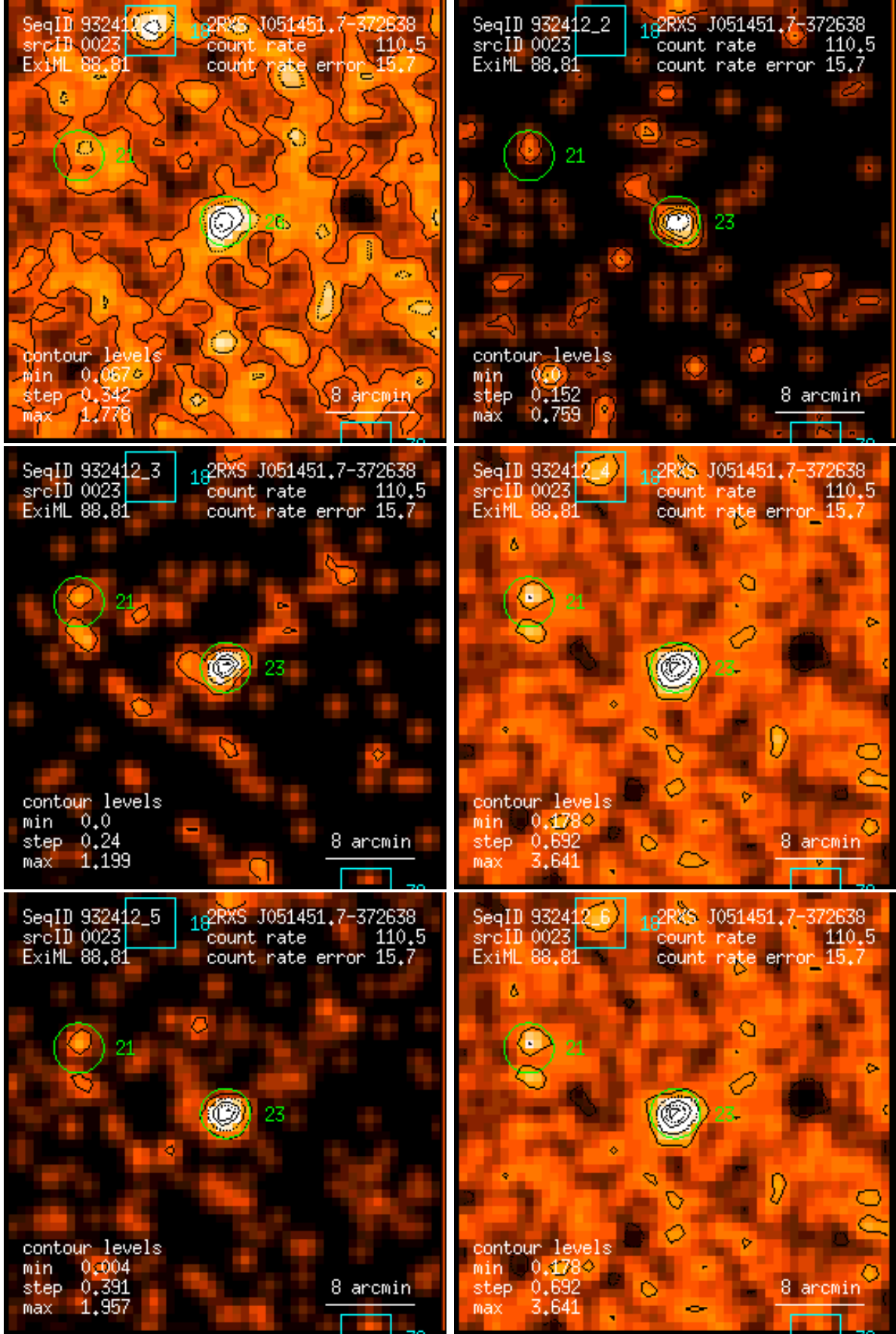
Figure 23: RASS 932412: detection 0023: band rate images, Gaussian filter: (1) PSPC channels 11 – 41, (2) 52 – 90, (3) 91 – 201, (4) 11 – 235, (5) 52 – 201, (6) 11 – 201. Broad band rates in counts/ks. Band rate contour levels in counts/ks/arcmin 2 .
