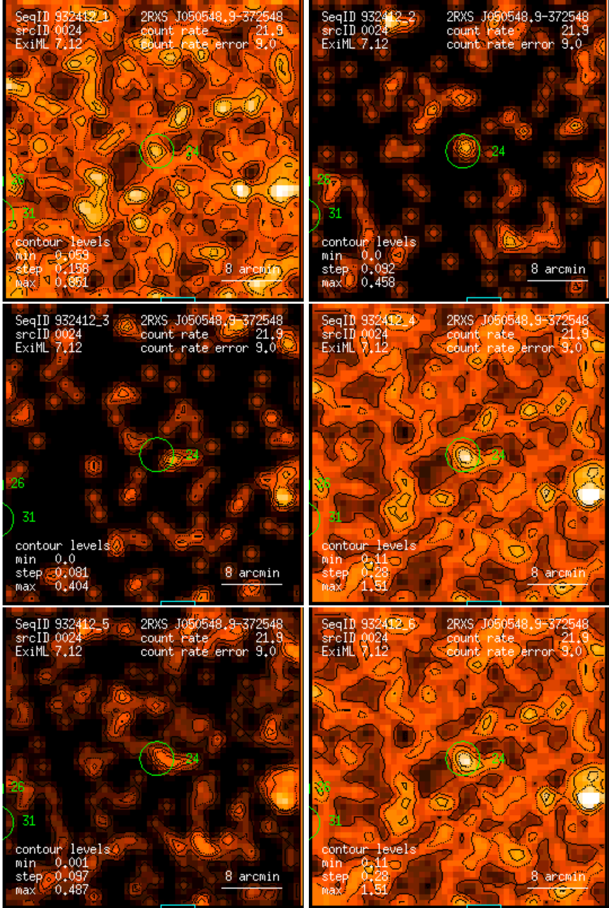
Figure 24: RASS 932412: detection 0024: band rate images, Gaussian filter: (1) PSPC channels 11 – 41, (2) 52 – 90, (3) 91 – 201, (4) 11 – 235, (5) 52 – 201, (6) 11 – 201. Broad band rates in counts/ks. Band rate contour levels in counts/ks/arcmin 2 .
