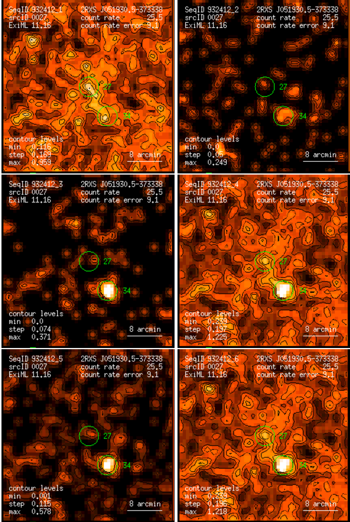
Figure 27: RASS 932412: detection 0027: band rate images, Gaussian filter: (1) PSPC channels 11 – 41, (2) 52 – 90, (3) 91 – 201, (4) 11 – 235, (5) 52 – 201, (6) 11 – 201. Broad band rates in counts/ks. Band rate contour levels in counts/ks/arcmin 2 .
