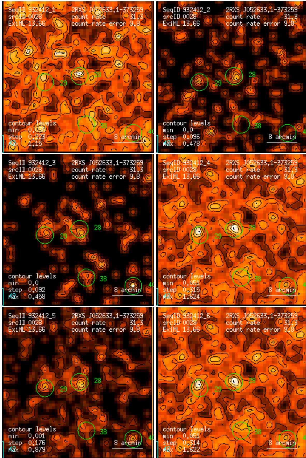
Figure 28: RASS 932412: detection 0028: band rate images, Gaussian filter: (1) PSPC channels 11 – 41, (2) 52 – 90, (3) 91 – 201, (4) 11 – 235, (5) 52 – 201, (6) 11 – 201. Broad band rates in counts/ks. Band rate contour levels in counts/ks/arcmin 2 .
