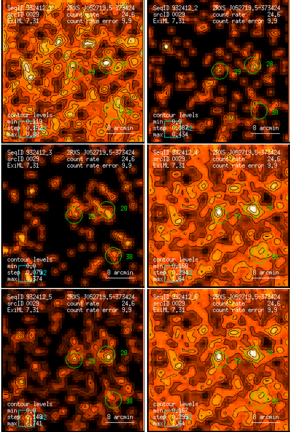
Figure 29: RASS 932412: detection 0029: band rate images, Gaussian filter: (1) PSPC channels 11 – 41, (2) 52 – 90, (3) 91 – 201, (4) 11 – 235, (5) 52 – 201, (6) 11 – 201. Broad band rates in counts/ks. Band rate contour levels in counts/ks/arcmin 2 .
