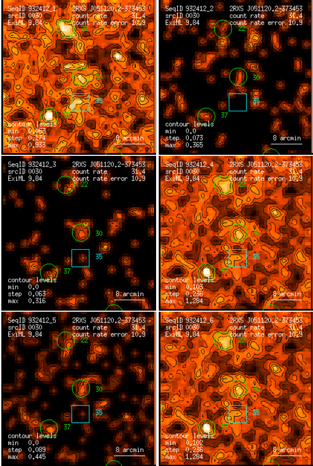
Figure 30: RASS 932412: detection 0030: band rate images, Gaussian filter: (1) PSPC channels 11 – 41, (2) 52 – 90, (3) 91 – 201, (4) 11 – 235, (5) 52 – 201, (6) 11 – 201. Broad band rates in counts/ks. Band rate contour levels in counts/ks/arcmin 2 .
