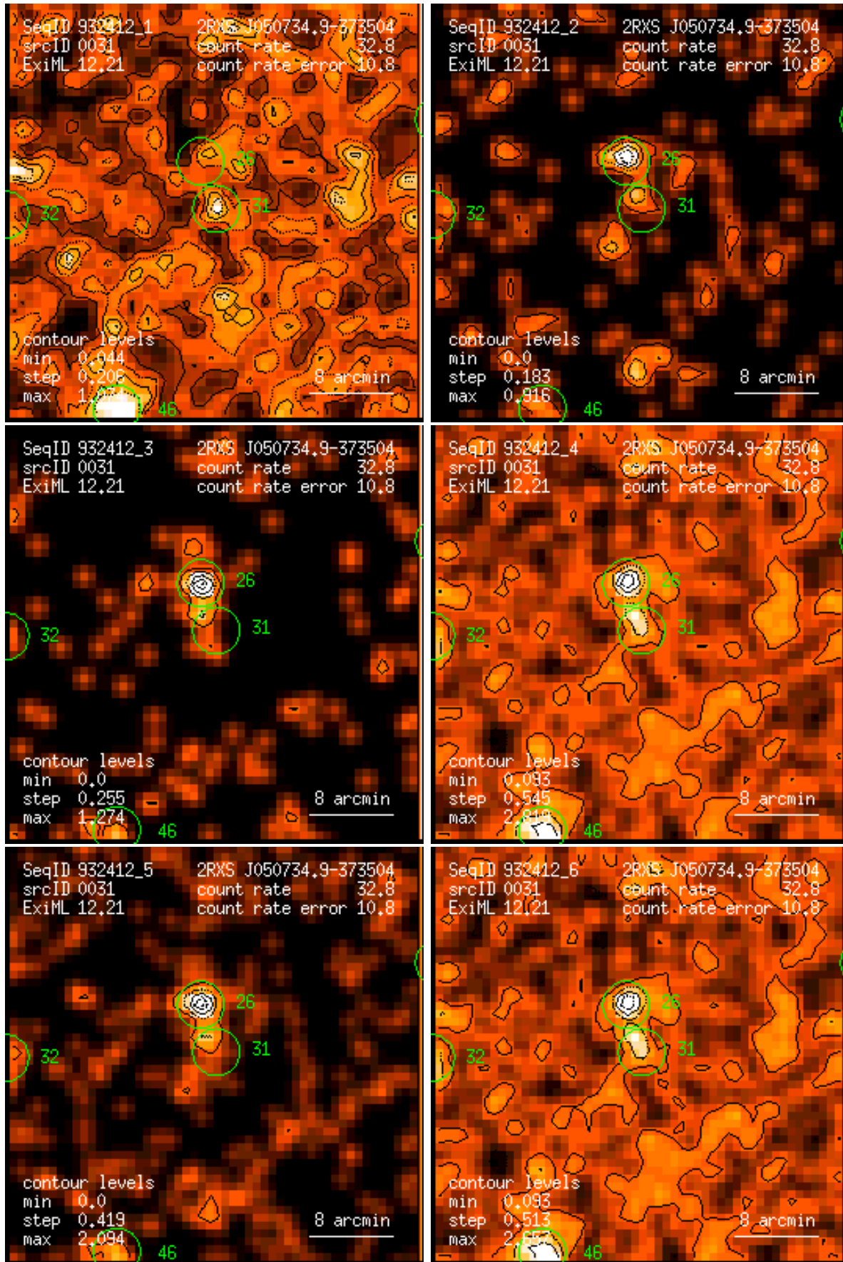
Figure 31: RASS 932412: detection 0031: band rate images, Gaussian filter: (1) PSPC channels 11 – 41, (2) 52 – 90, (3) 91 – 201, (4) 11 – 235, (5) 52 – 201, (6) 11 – 201. Broad band rates in counts/ks. Band rate contour levels in counts/ks/arcmin 2 .
