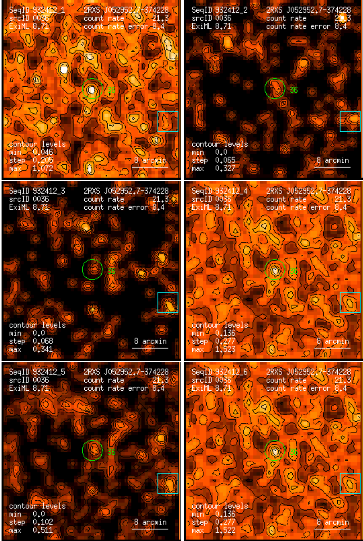
Figure 36: RASS 932412: detection 0036: band rate images, Gaussian filter: (1) PSPC channels 11 – 41, (2) 52 – 90, (3) 91 – 201, (4) 11 – 235, (5) 52 – 201, (6) 11 – 201. Broad band rates in counts/ks. Band rate contour levels in counts/ks/arcmin 2 .
