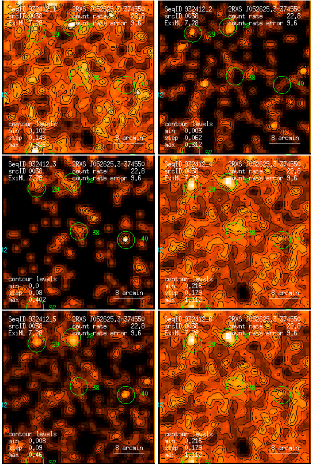
Figure 38: RASS 932412: detection 0038: band rate images, Gaussian filter: (1) PSPC channels 11 – 41, (2) 52 – 90, (3) 91 – 201, (4) 11 – 235, (5) 52 – 201, (6) 11 – 201. Broad band rates in counts/ks. Band rate contour levels in counts/ks/arcmin 2 .
