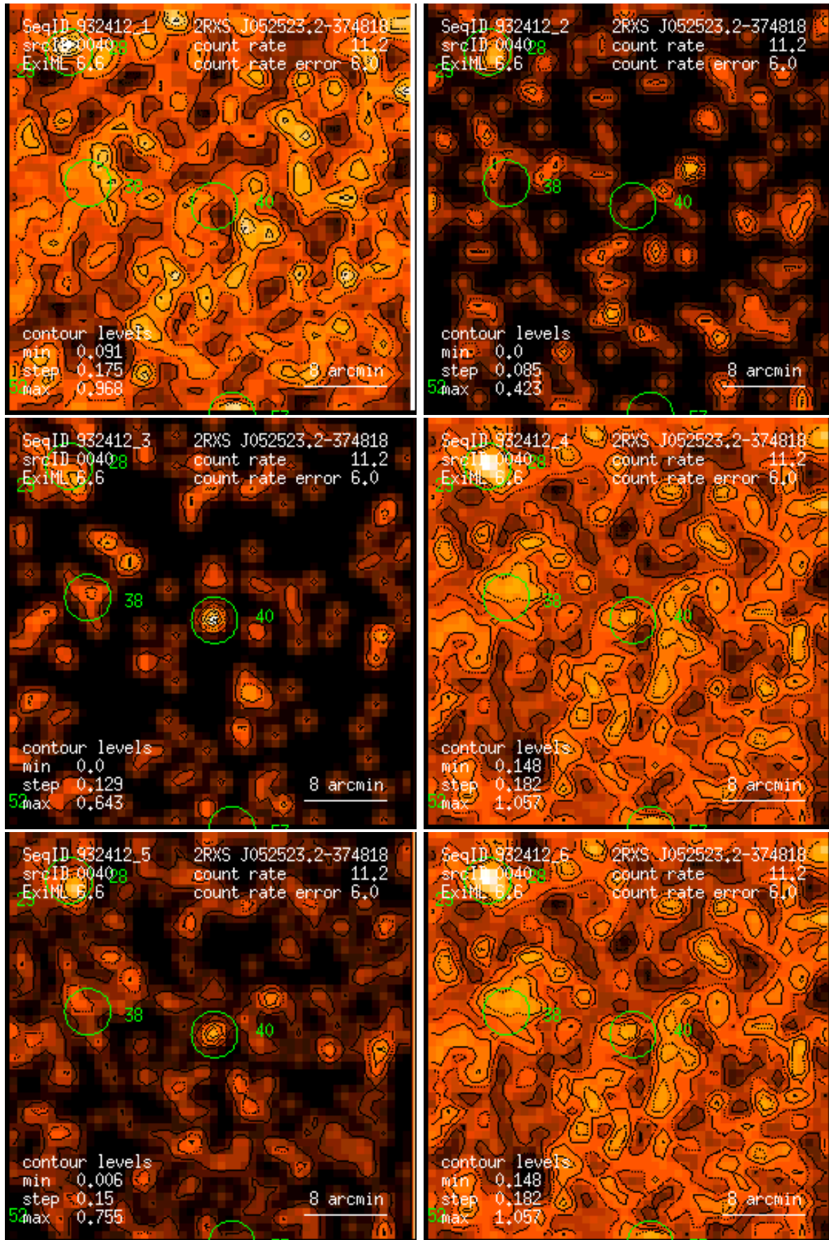
Figure 40: RASS 932412: detection 0040: band rate images, Gaussian filter: (1) PSPC channels 11 – 41, (2) 52 – 90, (3) 91 – 201, (4) 11 – 235, (5) 52 – 201, (6) 11 – 201. Broad band rates in counts/ks. Band rate contour levels in counts/ks/arcmin 2 .
