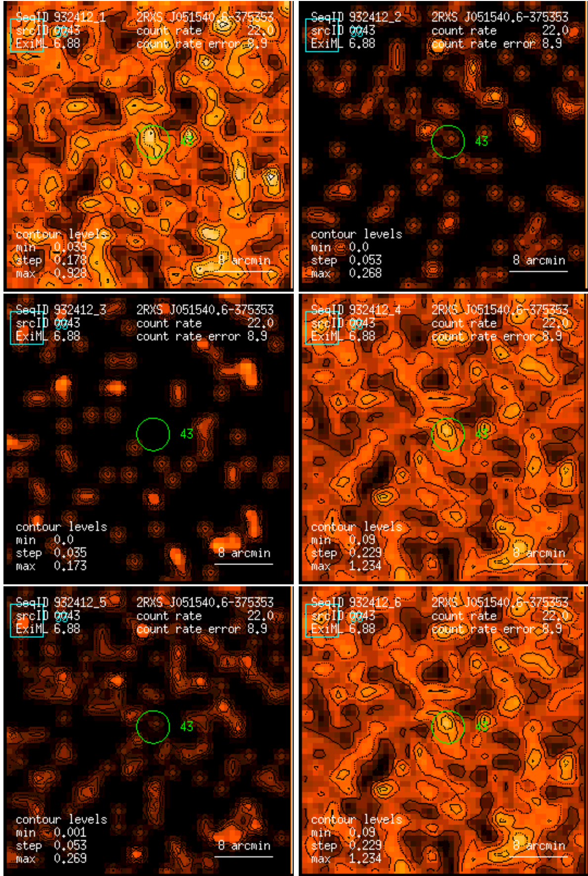
Figure 43: RASS 932412: detection 0043: band rate images, Gaussian filter: (1) PSPC channels 11 – 41, (2) 52 – 90, (3) 91 – 201, (4) 11 – 235, (5) 52 – 201, (6) 11 – 201. Broad band rates in counts/ks. Band rate contour levels in counts/ks/arcmin 2 .
