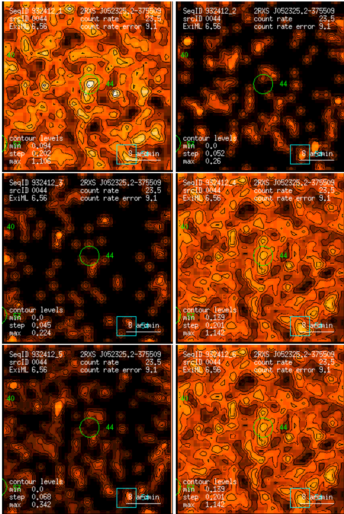
Figure 44: RASS 932412: detection 0044: band rate images, Gaussian filter: (1) PSPC channels 11 – 41, (2) 52 – 90, (3) 91 – 201, (4) 11 – 235, (5) 52 – 201, (6) 11 – 201. Broad band rates in counts/ks. Band rate contour levels in counts/ks/arcmin 2 .
