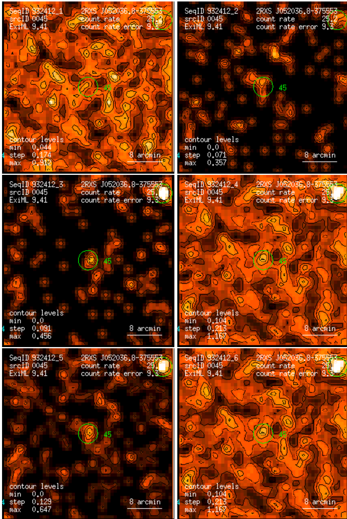
Figure 45: RASS 932412: detection 0045: band rate images, Gaussian filter: (1) PSPC channels 11 – 41, (2) 52 – 90, (3) 91 – 201, (4) 11 – 235, (5) 52 – 201, (6) 11 – 201. Broad band rates in counts/ks. Band rate contour levels in counts/ks/arcmin 2 .
