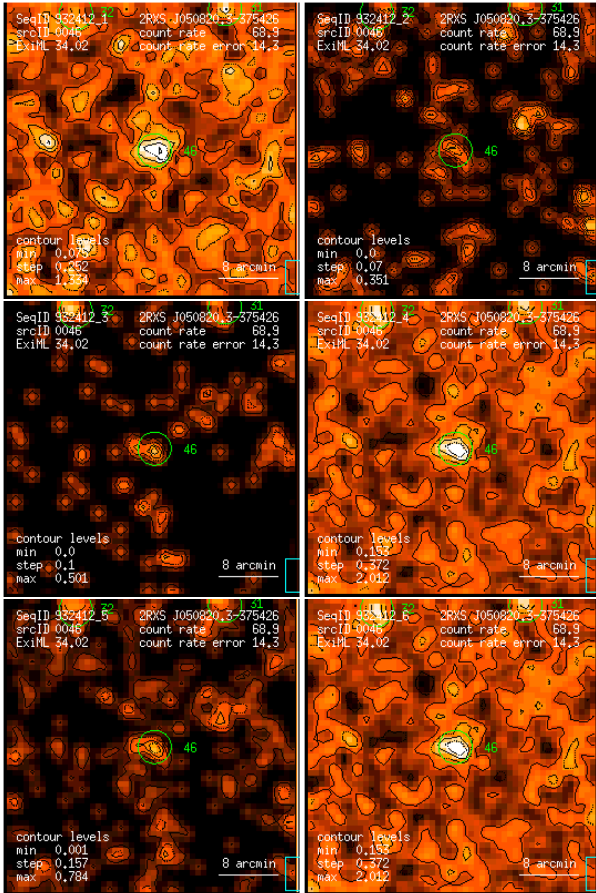
Figure 46: RASS 932412: detection 0046: band rate images, Gaussian filter: (1) PSPC channels 11 – 41, (2) 52 – 90, (3) 91 – 201, (4) 11 – 235, (5) 52 – 201, (6) 11 – 201. Broad band rates in counts/ks. Band rate contour levels in counts/ks/arcmin 2 .
