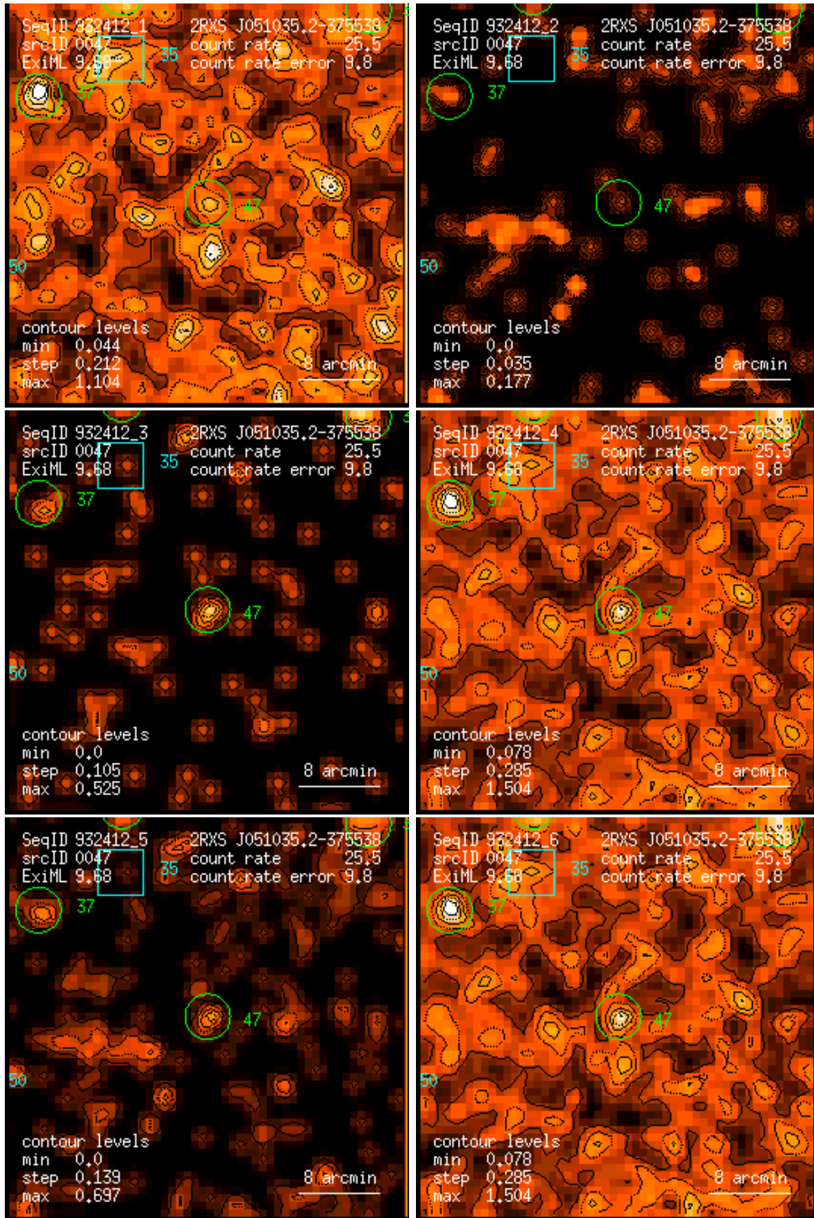
Figure 47: RASS 932412: detection 0047: band rate images, Gaussian filter: (1) PSPC channels 11 – 41, (2) 52 – 90, (3) 91 – 201, (4) 11 – 235, (5) 52 – 201, (6) 11 – 201. Broad band rates in counts/ks. Band rate contour levels in counts/ks/arcmin 2 .
