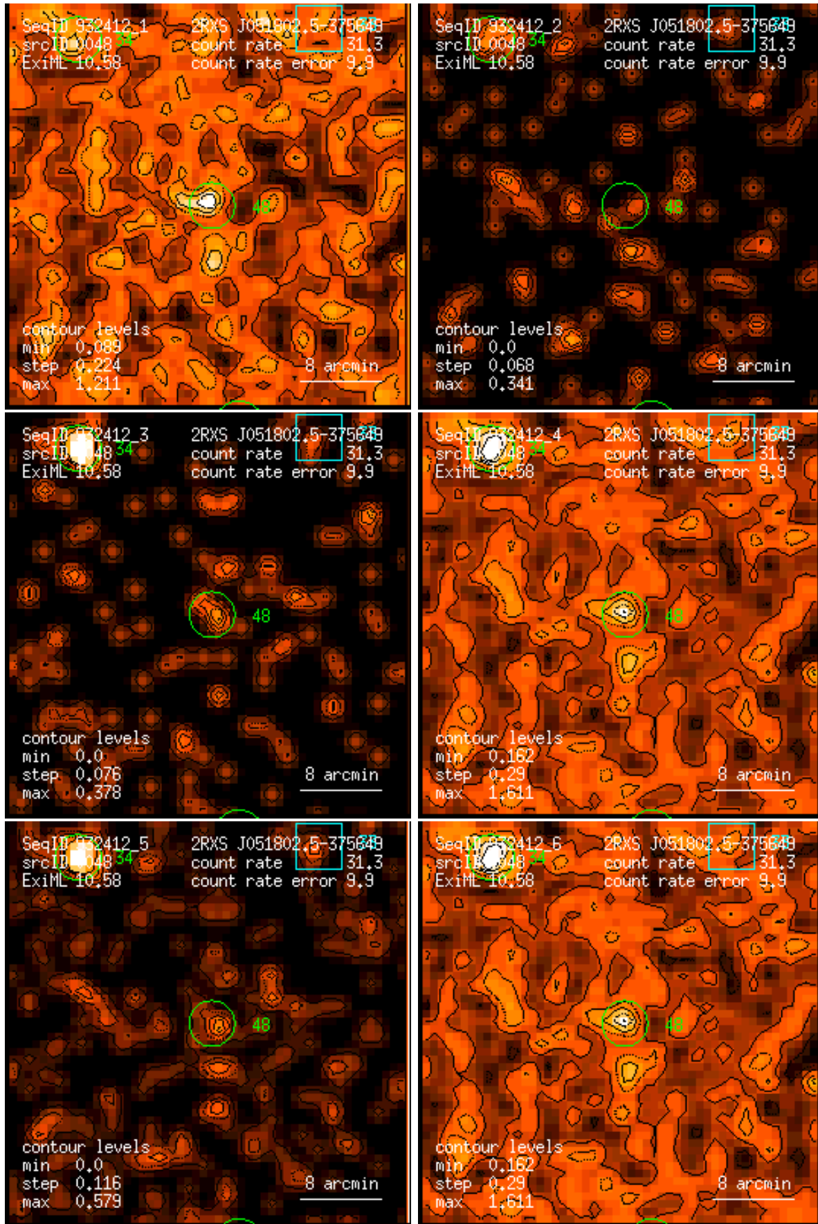
Figure 48: RASS 932412: detection 0048: band rate images, Gaussian filter: (1) PSPC channels 11 – 41, (2) 52 – 90, (3) 91 – 201, (4) 11 – 235, (5) 52 – 201, (6) 11 – 201. Broad band rates in counts/ks. Band rate contour levels in counts/ks/arcmin 2 .
