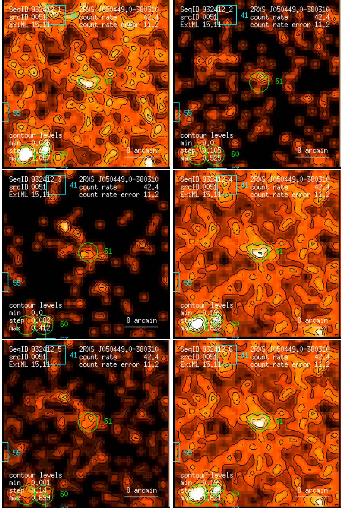
Figure 51: RASS 932412: detection 0051: band rate images, Gaussian filter: (1) PSPC channels 11 – 41, (2) 52 – 90, (3) 91 – 201, (4) 11 – 235, (5) 52 – 201, (6) 11 – 201. Broad band rates in counts/ks. Band rate contour levels in counts/ks/arcmin 2 .
