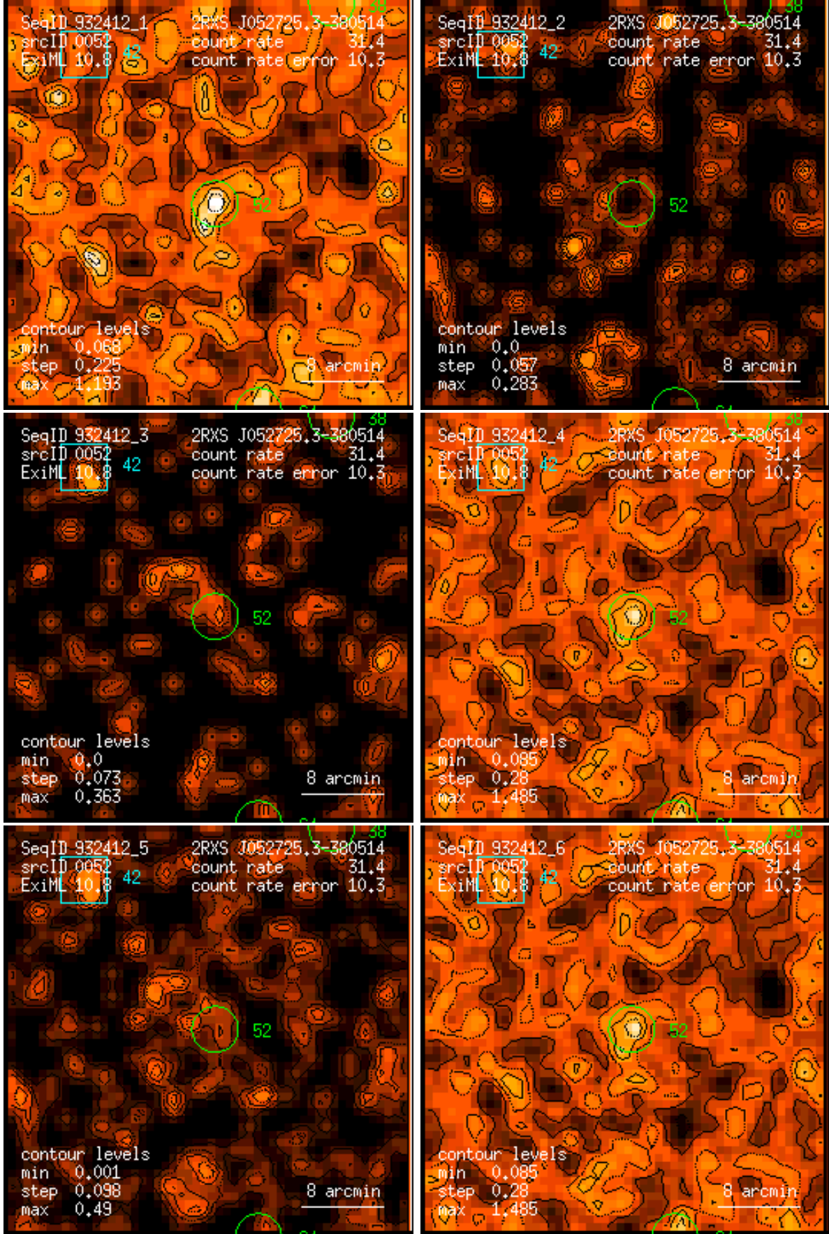
Figure 52: RASS 932412: detection 0052: band rate images, Gaussian filter: (1) PSPC channels 11 – 41, (2) 52 – 90, (3) 91 – 201, (4) 11 – 235, (5) 52 – 201, (6) 11 – 201. Broad band rates in counts/ks. Band rate contour levels in counts/ks/arcmin 2 .
