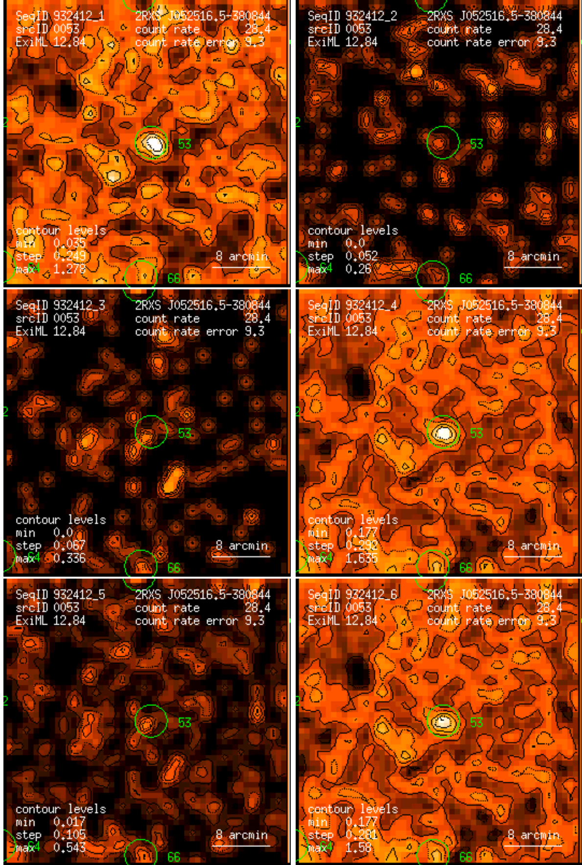
Figure 53: RASS 932412: detection 0053: band rate images, Gaussian filter: (1) PSPC channels 11 – 41, (2) 52 – 90, (3) 91 – 201, (4) 11 – 235, (5) 52 – 201, (6) 11 – 201. Broad band rates in counts/ks. Band rate contour levels in counts/ks/arcmin 2 .
