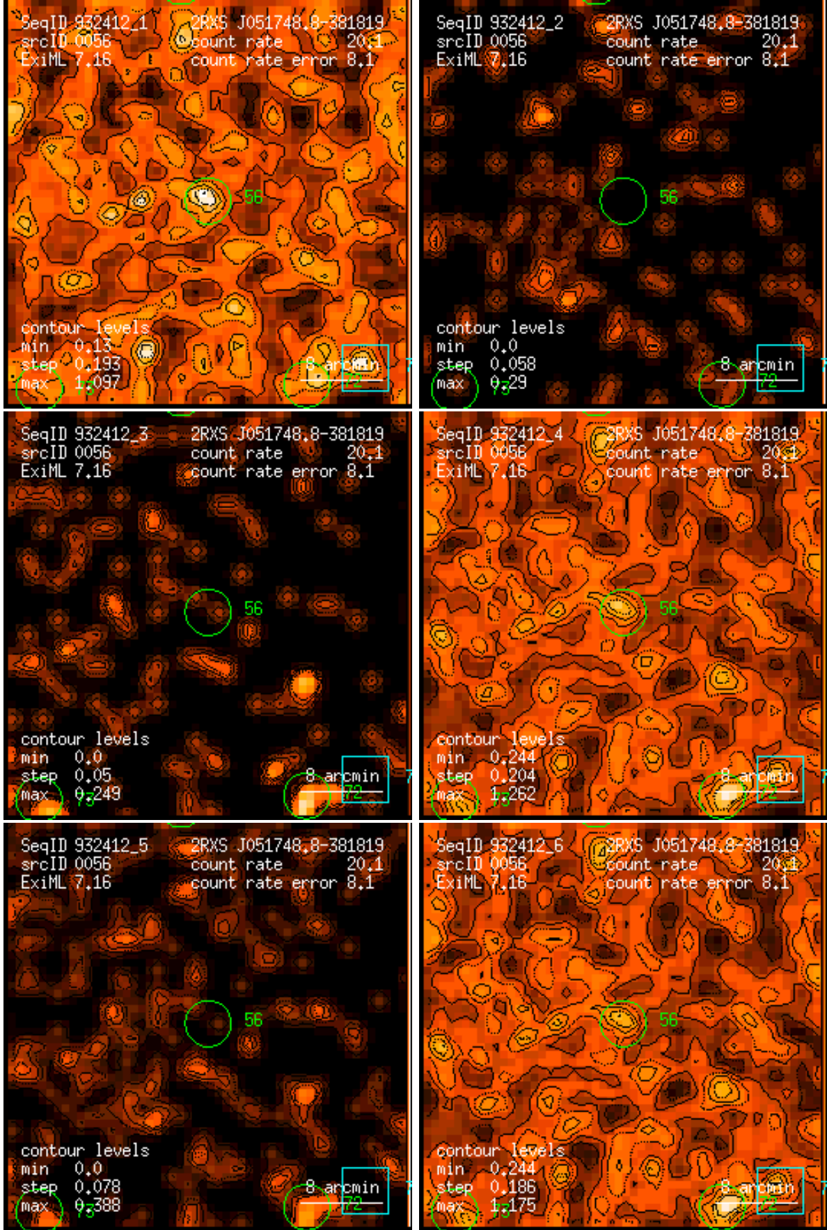
Figure 56: RASS 932412: detection 0056: band rate images, Gaussian filter: (1) PSPC channels 11 – 41, (2) 52 – 90, (3) 91 – 201, (4) 11 – 235, (5) 52 – 201, (6) 11 – 201. Broad band rates in counts/ks. Band rate contour levels in counts/ks/arcmin 2 .
