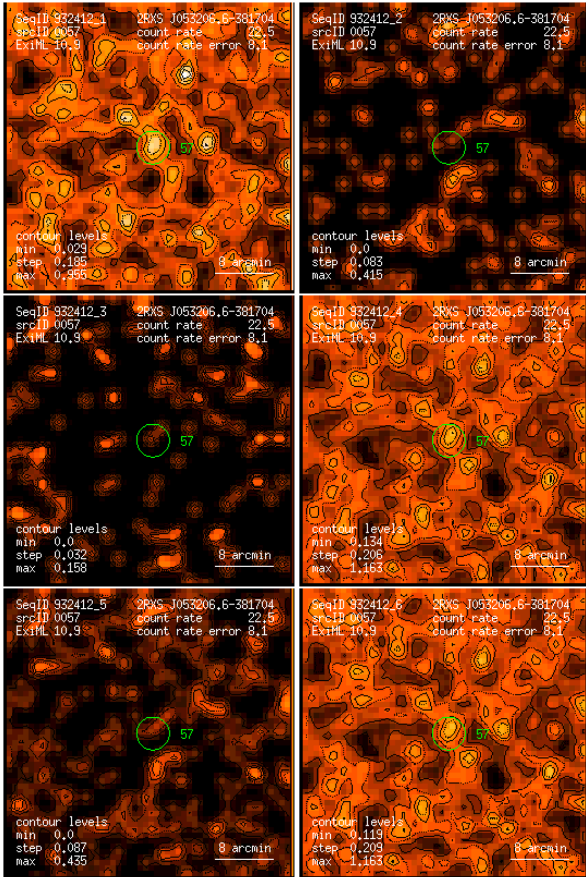
Figure 57: RASS 932412: detection 0057: band rate images, Gaussian filter: (1) PSPC channels 11 – 41, (2) 52 – 90, (3) 91 – 201, (4) 11 – 235, (5) 52 – 201, (6) 11 – 201. Broad band rates in counts/ks. Band rate contour levels in counts/ks/arcmin 2 .
