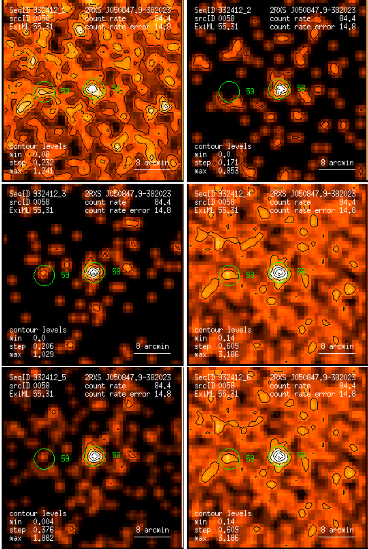
Figure 58: RASS 932412: detection 0058: band rate images, Gaussian filter: (1) PSPC channels 11 – 41, (2) 52 – 90, (3) 91 – 201, (4) 11 – 235, (5) 52 – 201, (6) 11 – 201. Broad band rates in counts/ks. Band rate contour levels in counts/ks/arcmin 2 .
