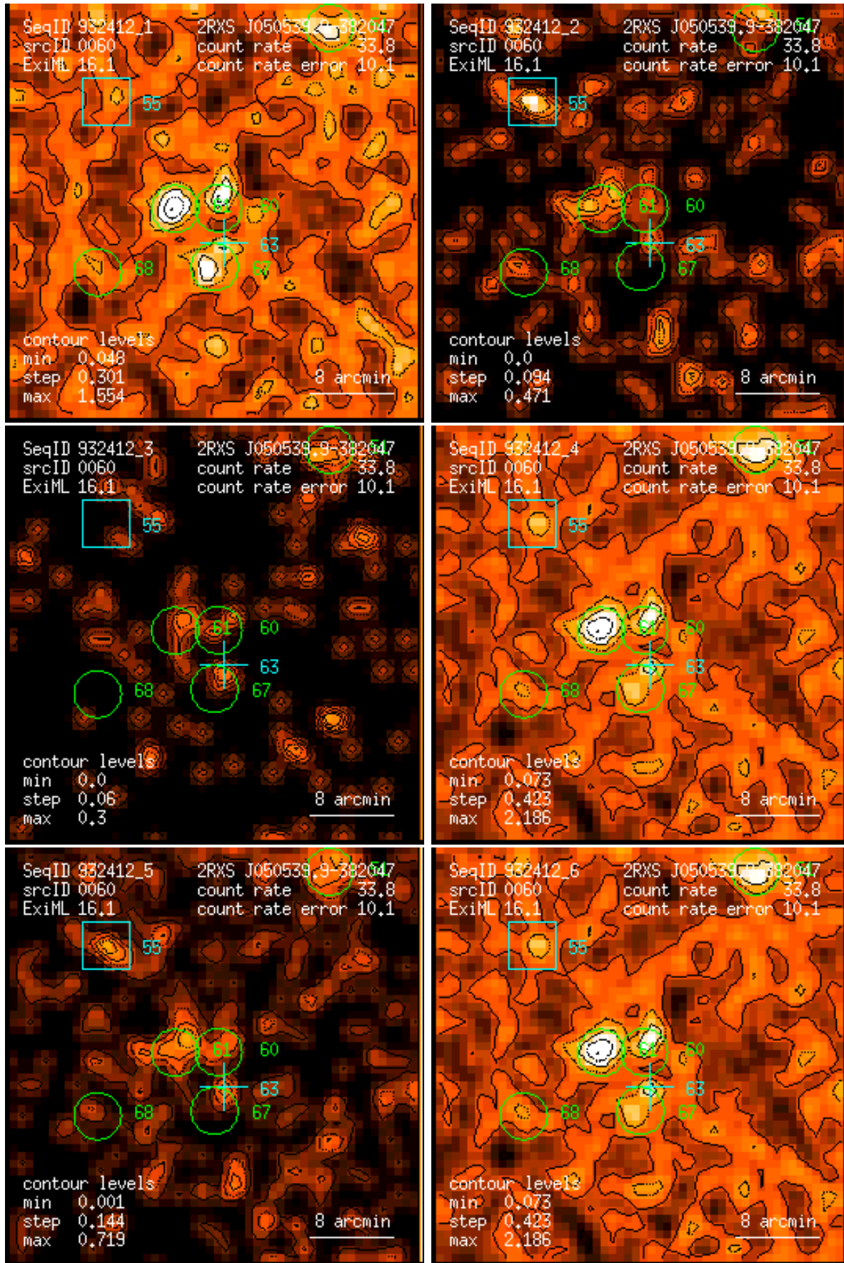
Figure 60: RASS 932412: detection 0060: band rate images, Gaussian filter: (1) PSPC channels 11 – 41, (2) 52 – 90, (3) 91 – 201, (4) 11 – 235, (5) 52 – 201, (6) 11 – 201. Broad band rates in counts/ks. Band rate contour levels in counts/ks/arcmin 2 .
