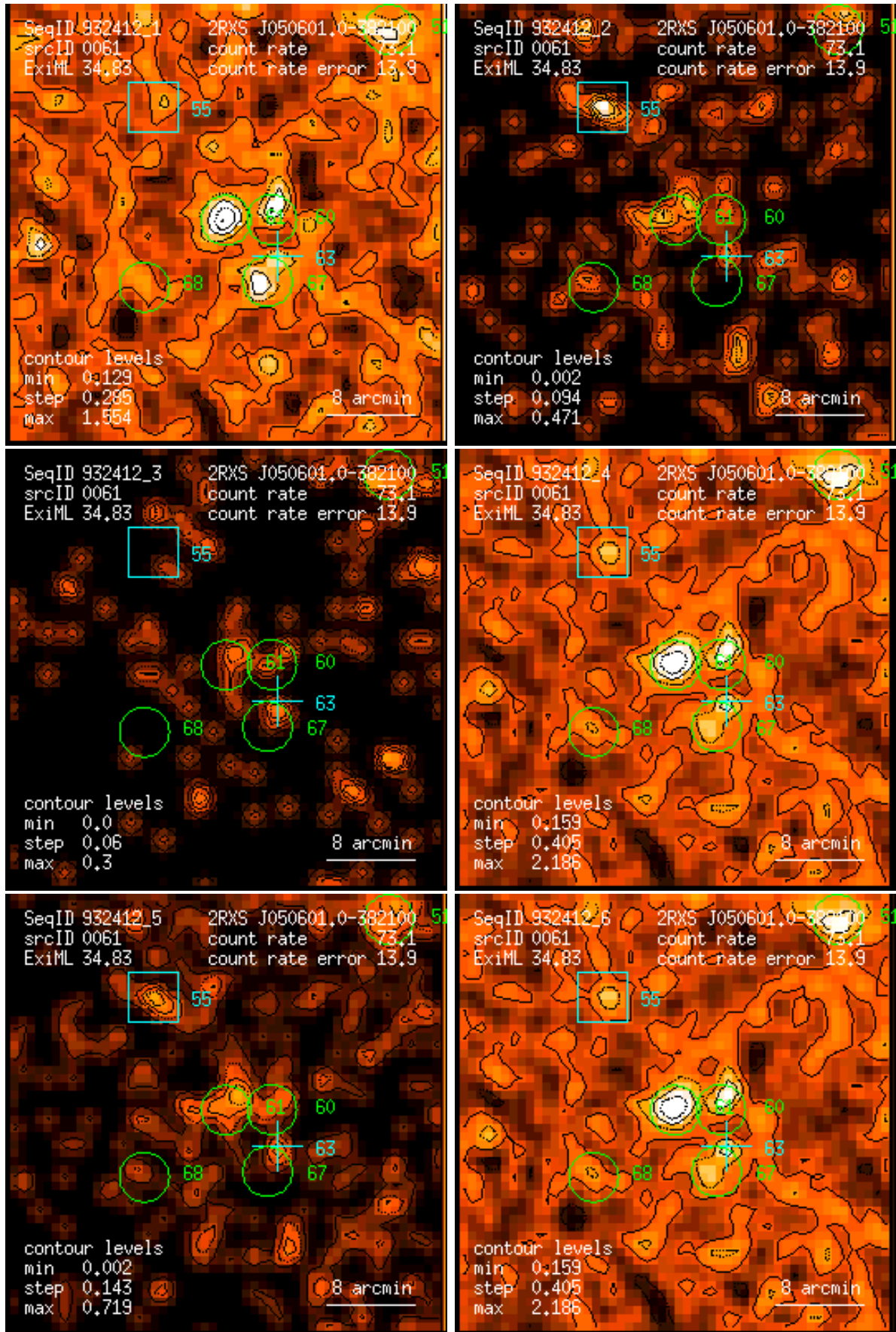
Figure 61: RASS 932412: detection 0061: band rate images, Gaussian filter: (1) PSPC channels 11 – 41, (2) 52 – 90, (3) 91 – 201, (4) 11 – 235, (5) 52 – 201, (6) 11 – 201. Broad band rates in counts/ks. Band rate contour levels in counts/ks/arcmin 2 .
