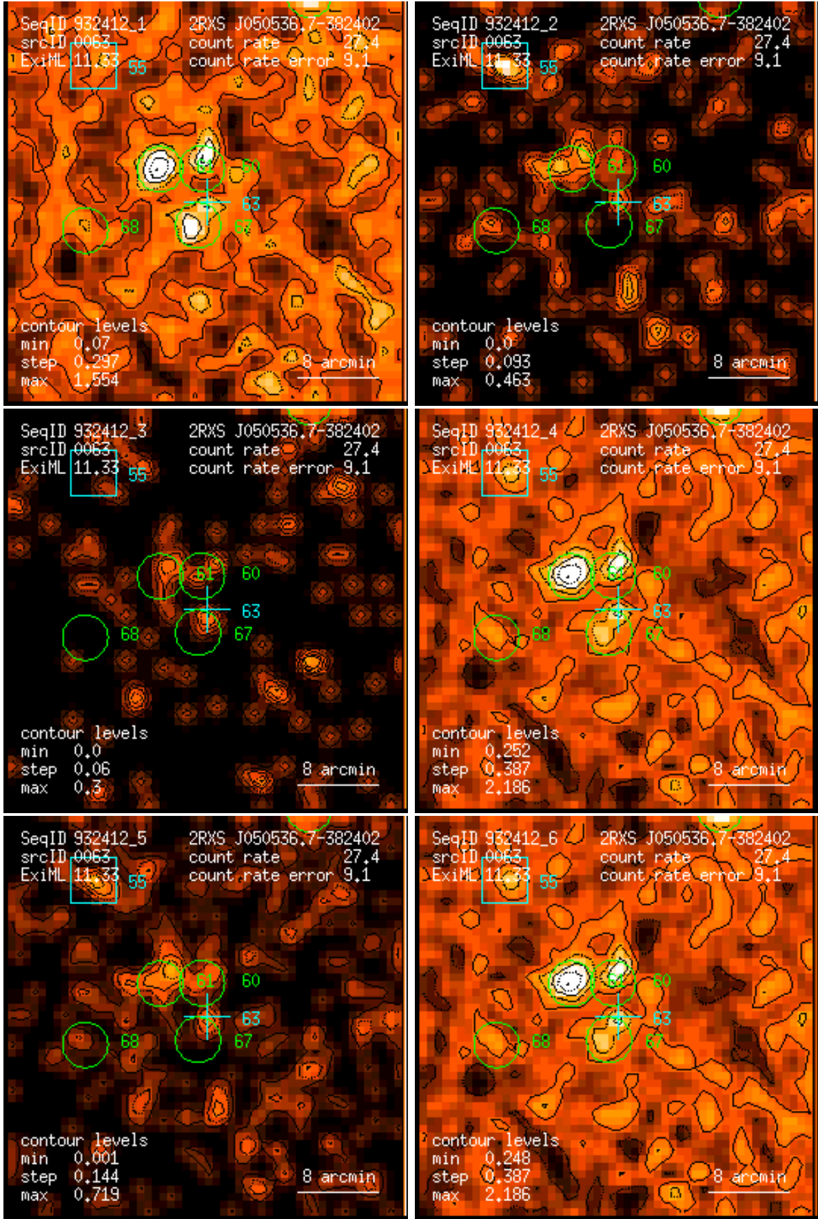
Figure 63: RASS 932412: detection 0063: band rate images, Gaussian filter: (1) PSPC channels 11 – 41, (2) 52 – 90, (3) 91 – 201, (4) 11 – 235, (5) 52 – 201, (6) 11 – 201. Broad band rates in counts/ks. Band rate contour levels in counts/ks/arcmin 2 .
