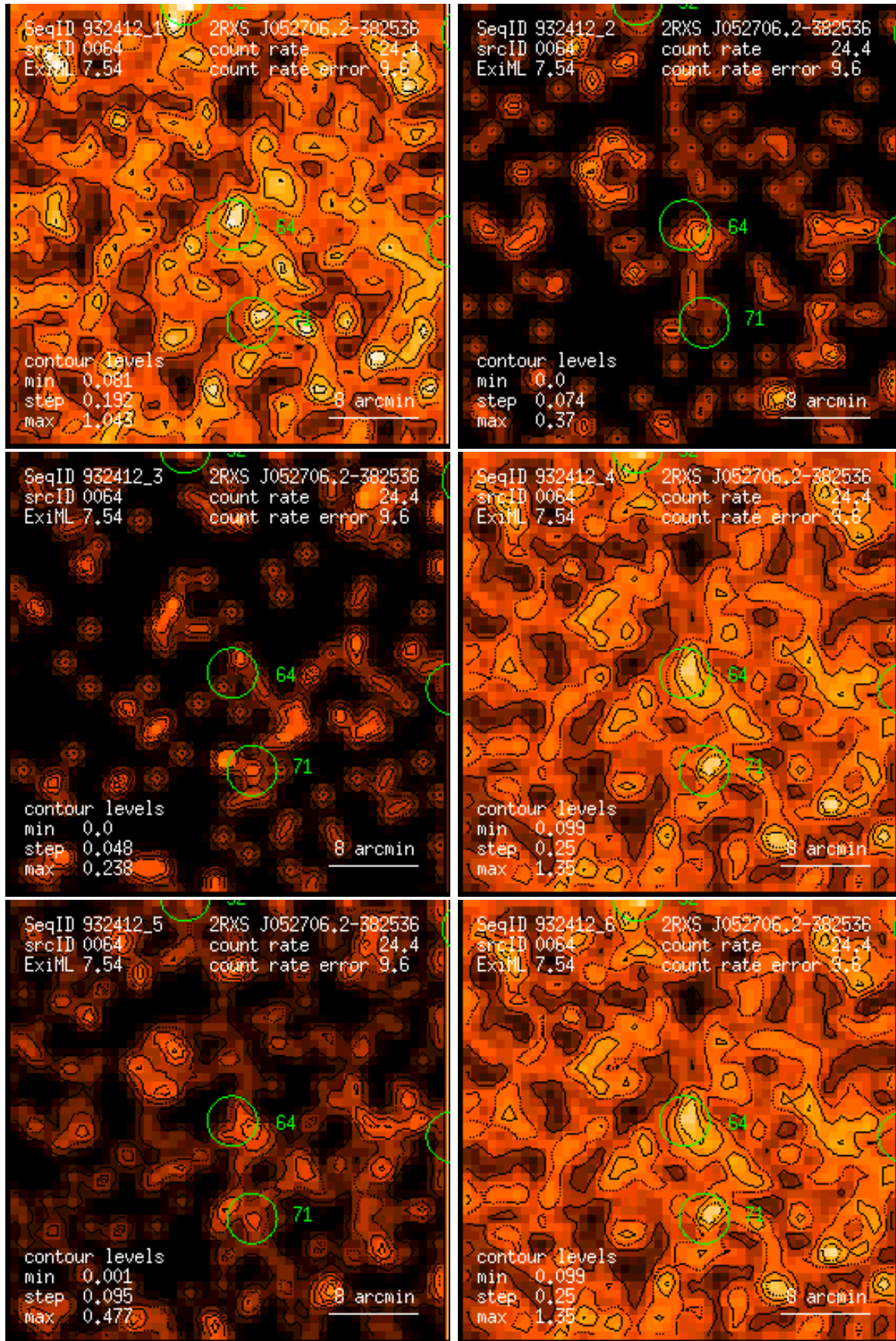
Figure 64: RASS 932412: detection 0064: band rate images, Gaussian filter: (1) PSPC channels 11 – 41, (2) 52 – 90, (3) 91 – 201, (4) 11 – 235, (5) 52 – 201, (6) 11 – 201. Broad band rates in counts/ks. Band rate contour levels in counts/ks/arcmin 2 .
