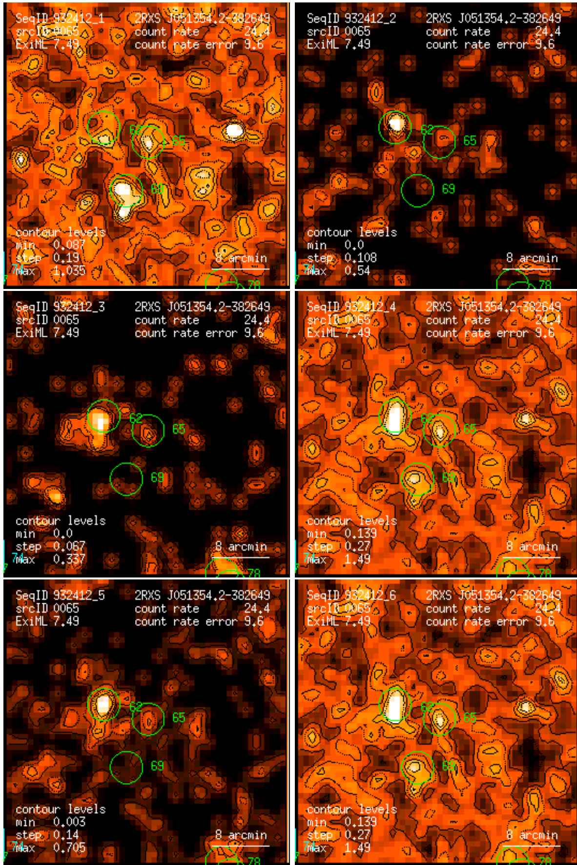
Figure 65: RASS 932412: detection 0065: band rate images, Gaussian filter: (1) PSPC channels 11 – 41, (2) 52 – 90, (3) 91 – 201, (4) 11 – 235, (5) 52 – 201, (6) 11 – 201. Broad band rates in counts/ks. Band rate contour levels in counts/ks/arcmin 2 .
