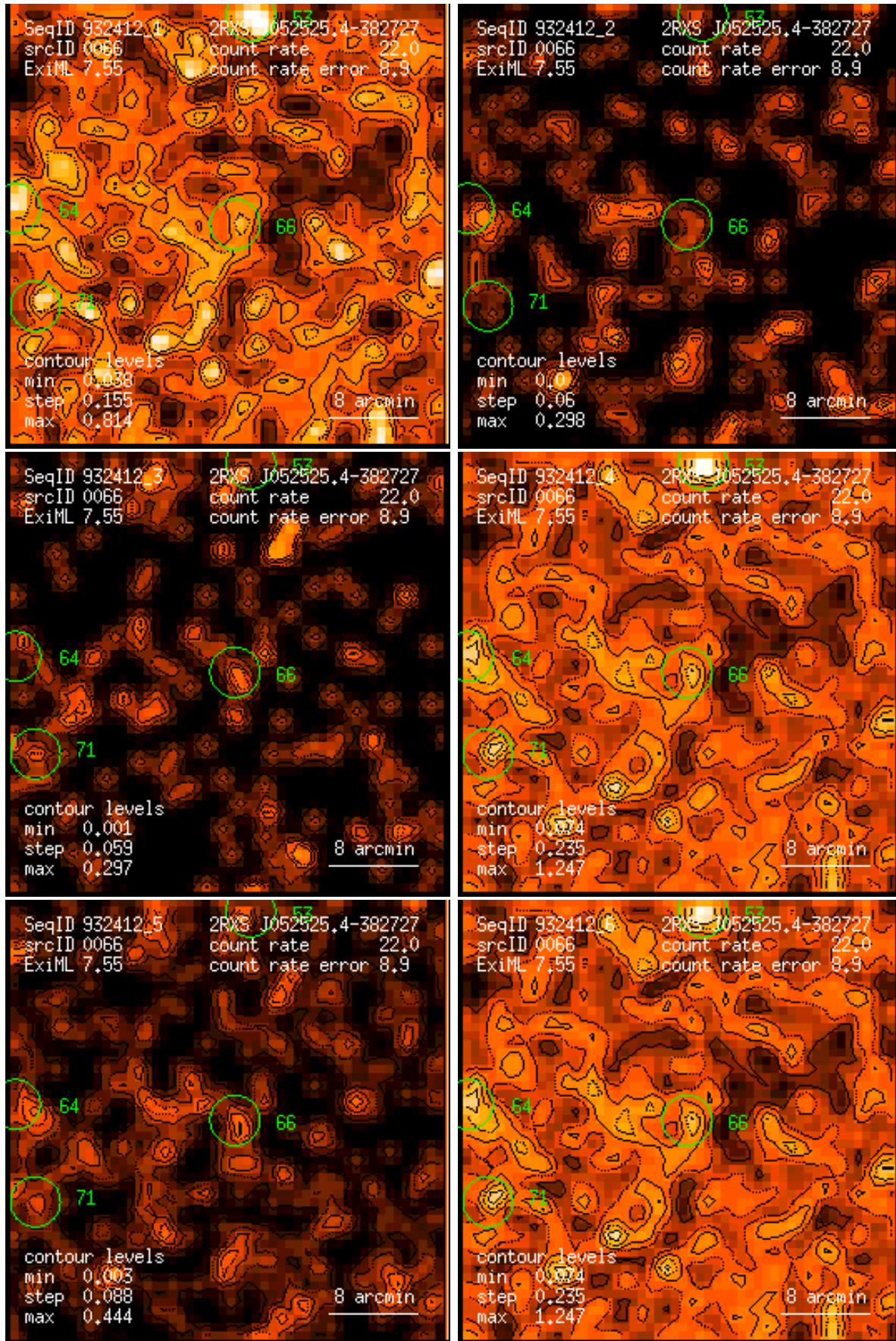
Figure 66: RASS 932412: detection 0066: band rate images, Gaussian filter: (1) PSPC channels 11 – 41, (2) 52 – 90, (3) 91 – 201, (4) 11 – 235, (5) 52 – 201, (6) 11 – 201. Broad band rates in counts/ks. Band rate contour levels in counts/ks/arcmin 2 .
