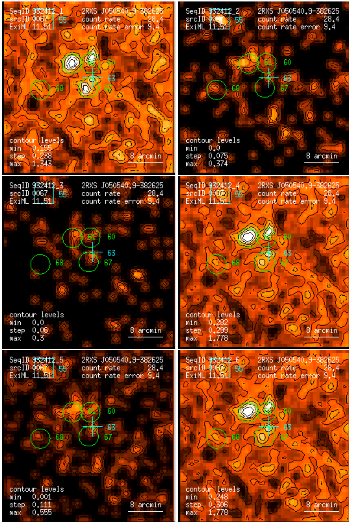
Figure 67: RASS 932412: detection 0067: band rate images, Gaussian filter: (1) PSPC channels 11 – 41, (2) 52 – 90, (3) 91 – 201, (4) 11 – 235, (5) 52 – 201, (6) 11 – 201. Broad band rates in counts/ks. Band rate contour levels in counts/ks/arcmin 2 .
