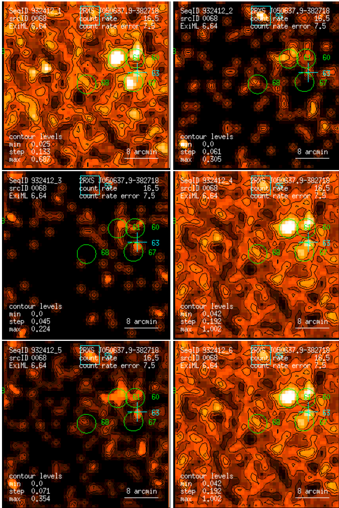
Figure 68: RASS 932412: detection 0068: band rate images, Gaussian filter: (1) PSPC channels 11 – 41, (2) 52 – 90, (3) 91 – 201, (4) 11 – 235, (5) 52 – 201, (6) 11 – 201. Broad band rates in counts/ks. Band rate contour levels in counts/ks/arcmin 2 .
